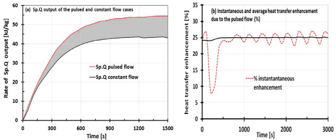
Figure 10 (a) Specific heat capacity of the radiators simulated at constant flow and pulsed flow (b) heat transfer enhancement of the radiator due the pulsed flow
