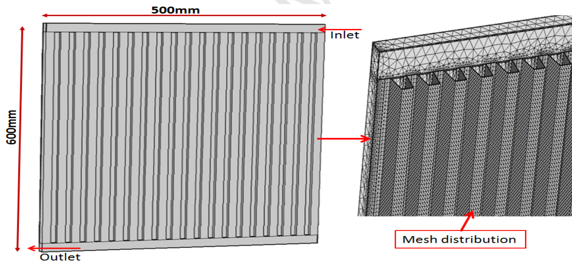
Figure 2 dimension and mesh distributions of the panel radiator
