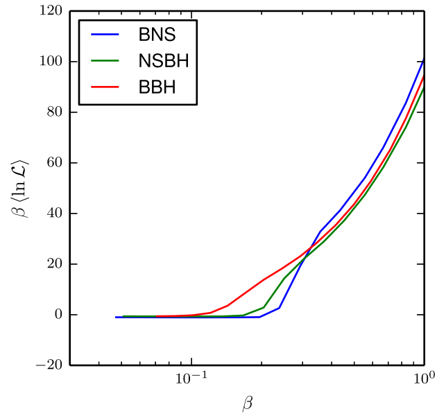
FIG. 5 (color online). The integrand of the evidence integral [Eq. (41)] versus \beta for the analyses of synthetic GW signals in § V B. The evidence is given by the area under each curve. Table I gives the results of the integration together with the estimated error in the quadrature, following the procedure described in § IV C. The jaggedness of the curves illustrates that the temperature spacing required for convergent MCMC simulations is larger than that required for accurate quadrature to compute the evidence; the flatness at small \beta illustrates that, for these simulations, the high-temperature limit is sufficient for convergence of the evidence integral.
