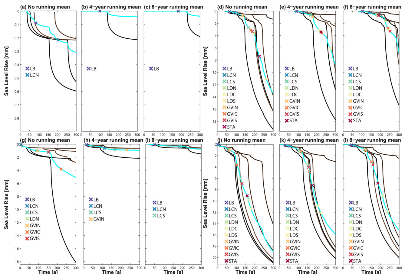
Figure 7. SLR curves to 2300, forced by using the -5°C isotherm (upper panel) and -9°C isotherm (lower panel) for emission scenarios RCP4.5 (left panel) and RCP8.5 (right panel). Crosses denote multimodel mean ice shelf collapse timings. Cyan line shows multimodel mean SLR curve.
