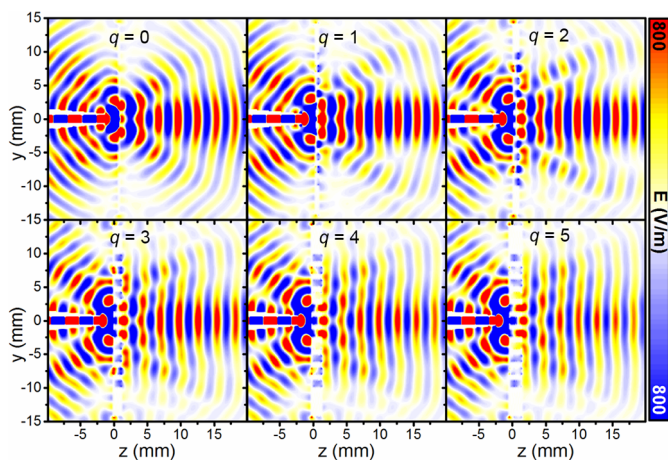
Figure 7 | Electric field distribution on the yz -plane. The colour-maps for the distribution of E_y component on the yz -plane for different number of stacked plates q .
