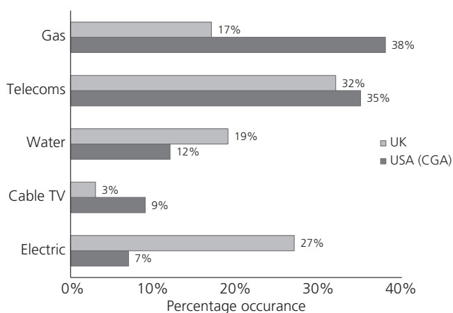
Figure 2. Percentage of all utility strikes by utility affected for the UK 3348 incidents and USA (CGA data, 208 000 incidents)
