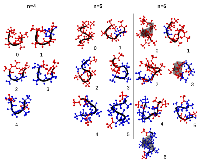
FIG. 1. Putative global minima obtained for the neutral alanine (Ace-(Ala) n -NHMe), ( n = 4, 5, 6 ) with chiralities systematically flipped on \alpha carbons. Blue atoms indicate atoms belonging to the D-Ala and red atoms correspond to L-Ala. Capping groups are also in red. The shaded regions indicate the helical nature of the backbone along with the sense of the helix.
