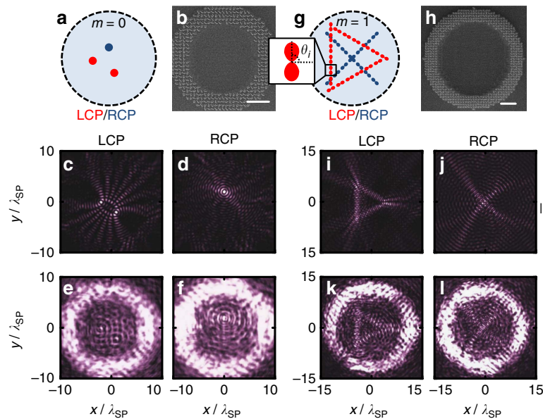
Figure 2 | Arbitrary spin-Hall effect. (a) Arbitrary spin splitting: LCP orbital to focus to two spots (red) while RCP orbital to focus a single spot (blue) (see text for detailed specification). (b) Top-view SEM image of the fabricated sample: a ring of nano-slots (with radii from 6.6\lambda_{SP} to 10\lambda_{SP} , embedded with a square array of particles separated by a = 2\lambda_{SP}/3 ). (c–f) are simulated |E_z|^2 and experimental intensity profiles for LCP and RCP incidence. (g) Arbitrary spin-dependent SPP profiles with more complicated pattern: shining LCP generating a triangle pattern (red) and shining RCP generating a cross pattern (blue). (h) Top-view SEM image of the fabricated sample (with radii from 10\lambda_{SP} to 13.3\lambda_{SP} and a = 2\lambda_{SP}/3 ). (i–l) simulated |E_z|^2 and experimental intensity profiles for LCP and RCP incidence. Here we use same colour scales for different incident CP. Scale bars, 4\mu\text{m} in b,h respectively.
