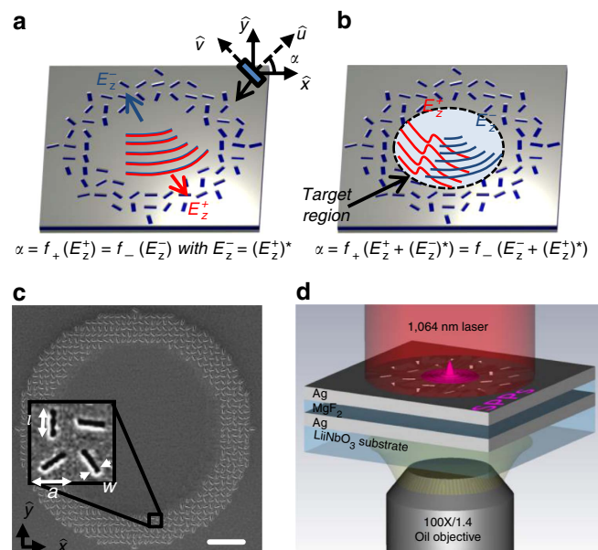
Figure 1 | Arbitrary OSHE of SPP. (a,b) Identical nano-slots with orientation profile \alpha(x,y) on the x-y plane with \hat{u}, \hat{v} as the local principal axes of each particle. Light is incident normally on the surface. \alpha can be designed by (a) direct substitution of the target SPP orbital E_z^{+}/E_z^{-} (for LCP and RCP incident wave) into equation (1) with restriction E_z^{+} = (E_z^{-})^* ; or (b) the modified matching rule equation (2) employed in this work to gain independent control of local SPP orbitals generated within the ring of nano-slots. (c) Top-view scanning electron microscopy (SEM) image of experiment sample. The sample is with geometrical parameters defined as l = 500 nm, w = 50 nm and a = 706 nm. Scale bars, 4 \mu\text{m} in (c). (d) Schematics of the experimental set-up.
