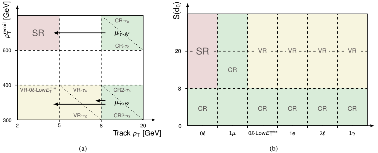
Figure 5: Schematics illustrating the selection of the CRs and VRs used to estimate (a) the tau track background and (b) the QCD track background, along with the orthogonality with respect to the SR. The arrows in (a) indicate the direction of extrapolation in the kinematic phase space which is validated in the VRs.
