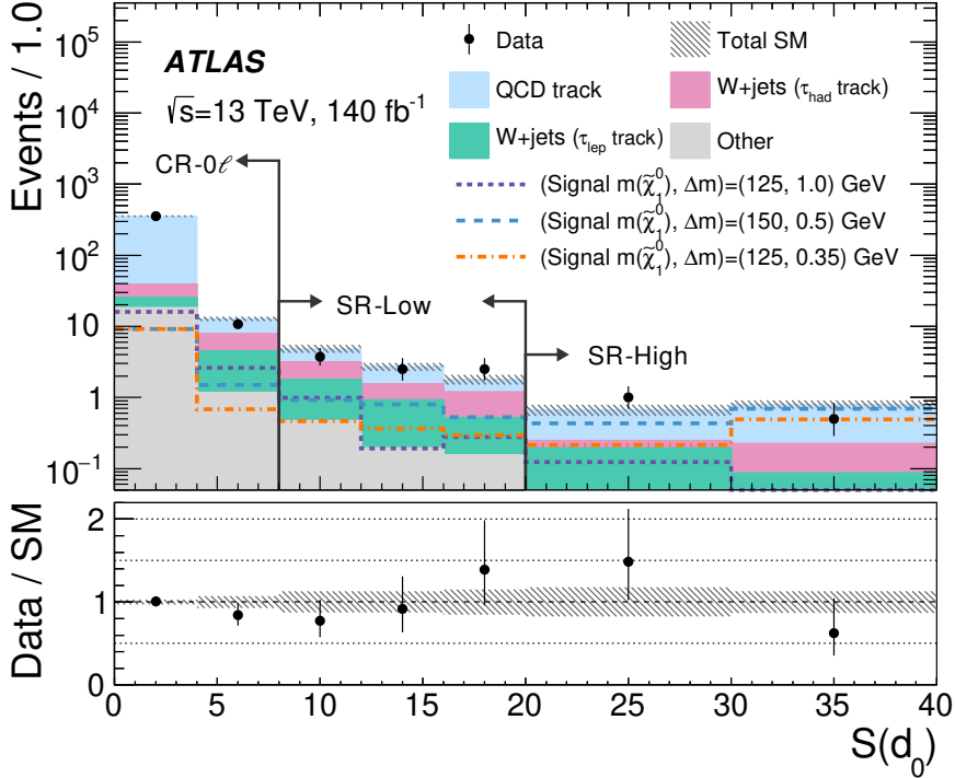
Figure 2: Post-fit S(d_0) distribution in the signal region bins and the adjacent control region (CR-0 \ell ), with the boundaries indicated by arrows. The SM background expectation is shown as a histogram stack, and a few representative signal models are overlaid. The last bin includes the overflow. The hatched band indicates the total uncertainty on the SM background expectation, including both statistical and systematic uncertainties.
