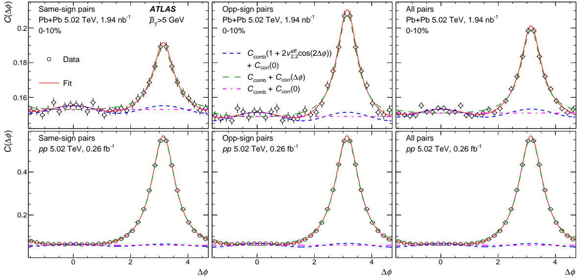
Figure 1: Measured two-muon correlation functions, C(\Delta\phi) . Top row: results for Pb+Pb data in the 0–10% centrality interval; Bottom row: pp results. Left column: same-sign pairs, Middle column: opposite-sign pairs, Right column: all pairs. Also shown are the results of fits of the correlation functions to Eq. (1), along with different components of the fits.
