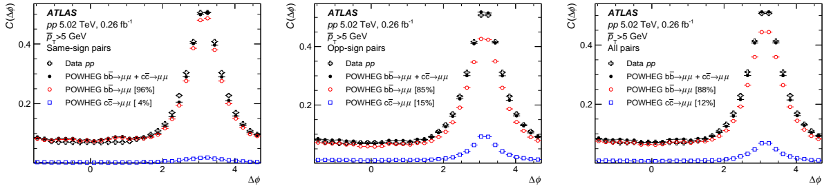
Figure 4: Correlation functions, C(\Delta\phi) , in the POWHEG+PYTHIA8 MC sample used in Figure 3. The left, center and right panels correspond to same-sign, opposite-sign and all-pairs respectively. The relative contribution of b\bar{b} and c\bar{c} pairs are also shown. The measured C(\Delta\phi) in the pp data are also shown for comparison.
