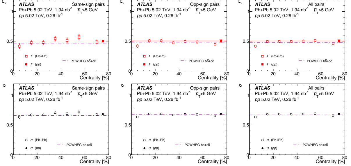
Figure 3: Comparison of the \Gamma (top) and \sigma (bottom) obtained from a POWHEG+PYTHIA8 MC sample to those obtained in the data. The horizontal continuous lines indicate the nominal pp values plotted across the full centrality range. The POWHEG+PYTHIA8 calculation includes two samples: a b\bar{b} \rightarrow \mu\mu and a c\bar{c} \rightarrow \mu\mu sample. The same fiducial selections are applied on the single-muons and on the muon-pair as those in the data analysis; namely that the single-muon |\eta| < 2.4 and p_T > 4 GeV, and that for the pair, \bar{p}_T > 5 GeV and |\Delta\eta| > 0.8 . The b\bar{b} and c\bar{c} samples are combined appropriately weighted by the cross-sections. The samples are generated using the nCTEQ15+SIH [74] nuclear PDFs corresponding to the Pb-nucleus, and thus include the correct admixture of pp , pn and nn collisions for comparison to the Pb+Pb measurements. The left, center and right panels correspond to same-sign, opposite-sign and all-pairs respectively.
