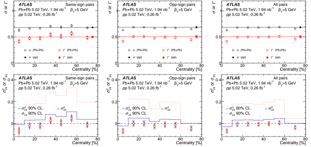
Figure 2: Top panels: The measured widths, \sigma , of the away-side peak in the two-particle correlation functions in Pb+Pb collisions versus centrality. Also shown are the values of the \Gamma parameter in Eq. (1). The \sigma and \Gamma measured in pp collisions are also shown. The vertical lines and shaded bands on the data points represent the statistical uncertainties, and systematic uncertainties, respectively. The horizontal lines indicate the nominal pp values plotted across the full centrality range. Bottom panels: The difference between the squared-widths of the Pb+Pb and pp measurements. Also shown are the upper limit on \sigma_{\text{int}}^2 and \sigma_{\text{int}} at the 90% CL. As the 90% CL on \sigma_{\text{int}}^2 is negative for the 0–10% centrality interval, the corresponding 90% CL on \sigma_{\text{int}} cannot be evaluated, and is not shown. The left, middle, and right panels correspond to same-sign pairs, opposite-sign pairs, and all-pairs.
