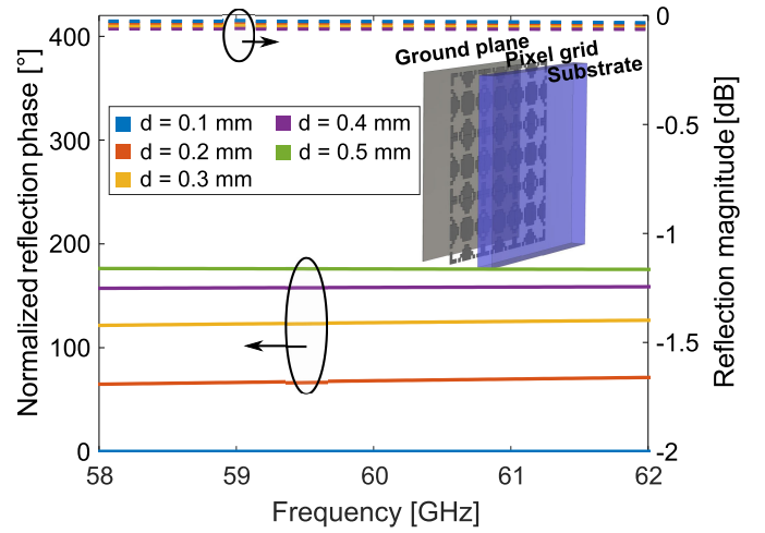
Fig. 6. Simulated performance of the selected solution. Normalized phase (solid lines) and magnitude (dashed lines) of the reflected wave for different ground plane displacements.
