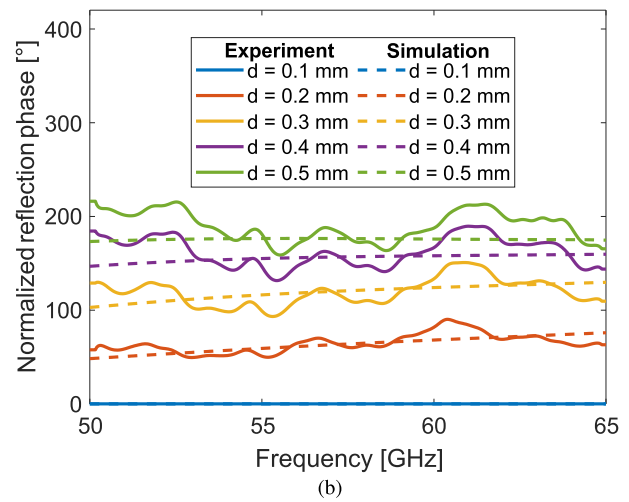
Fig. 10. Simulated and experimental results between 50 and 65 GHz for different displacements of the ground plane. (a) Reflection amplitude. (b) Normalized reflection phase.
