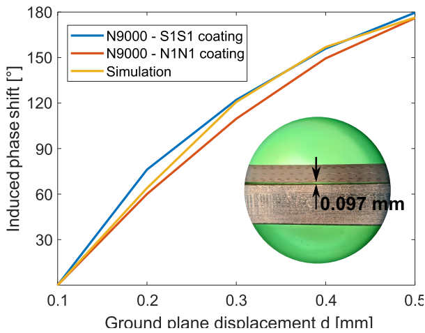
Fig. 11. Induced phase shift w.r.t ground plane displacement at center frequency (57.5 GHz). Experimental results of the two fabricated prototypes versus simulation and microscope illustration of the structure touching the ground plane.
