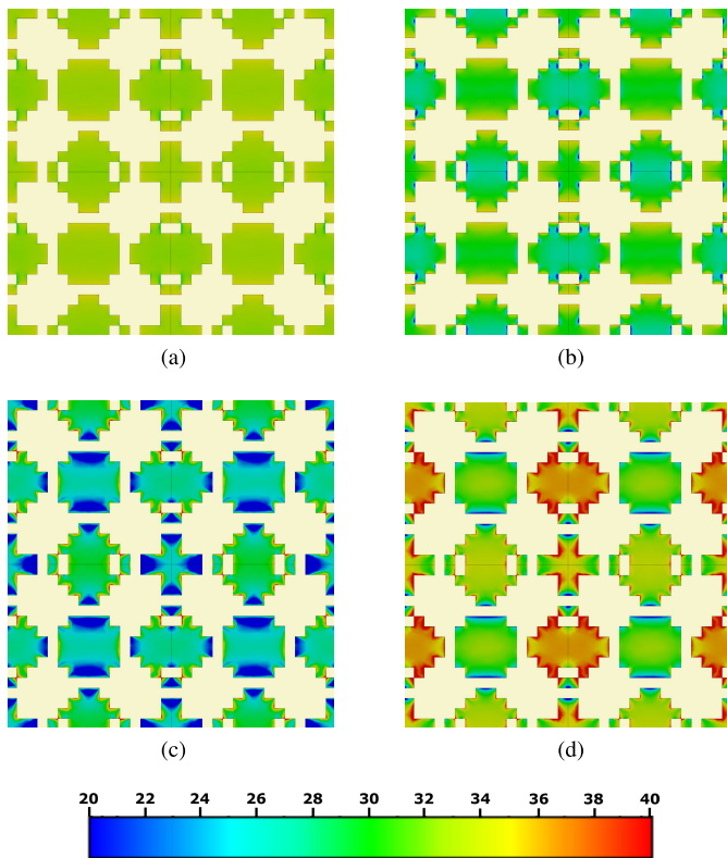
Fig. 13. Surface current distribution on the pixel grid of the metasurface for different frequencies and ground plane displacements. Units are in dB(A/m) (a) d = 0.1 mm @50 GHz. (b) d = 0.1 mm @65 GHz. (c) d = 0.5 mm @50 GHz. (d) d = 0.5 mm @65 GHz.
