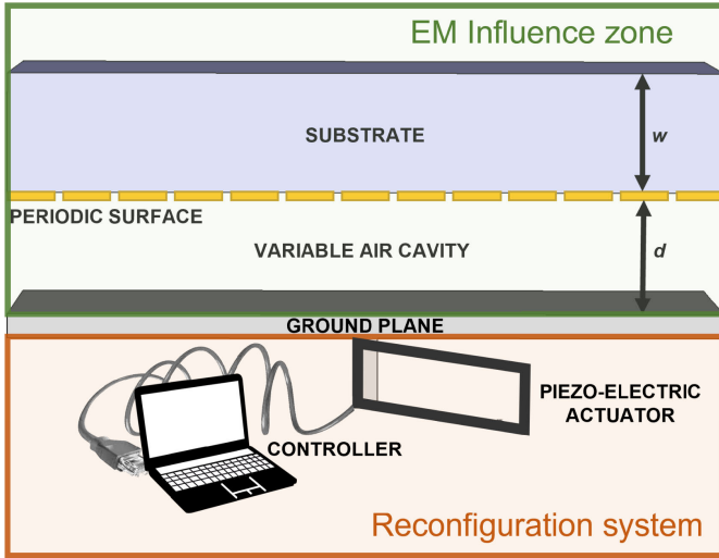
Fig. 2. Schematic of the proposed tunable phase shifter.
