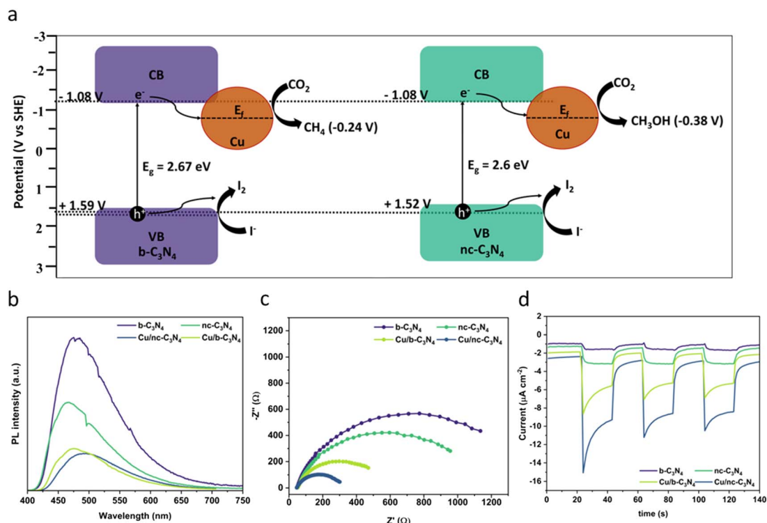
Fig. 5 (a) Proposed mechanism for \text{CO}_2 reduction showing the different band alignments for b\text{-C}_3\text{N}_4 and nc\text{-C}_3\text{N}_4 derived from Fig. S9–S11 † ( -0.87 V vs. \text{AgCl}/\text{Ag} corresponds to -1.08 V vs. SHE). (b) PL spectra (excitation = 445 nm) showing decreasing emission with increased graphitisation and Cu loading. (c) EIS measurements of carbon nitride materials with and without Cu. (d) Photocurrent response showing increasing concentration of charge carriers formed due to light absorption in the following order \text{Cu}/nc\text{-C}_3\text{N}_4 (dark blue) > \text{Cu}/b\text{-C}_3\text{N}_4 (light green) > nc\text{-C}_3\text{N}_4 (dark green) > b\text{-C}_3\text{N}_4 (purple).
