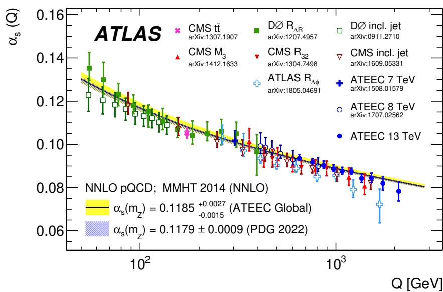
Figure 11. Comparison of the values of \alpha_s(Q) determined from fits to the ATEEC functions with the QCD prediction using the world average as input (hatched band) and the value obtained from the global fit (solid band). Results from previous analyses, both from ATLAS and from other experiments, are also included, showing an excellent agreement with the current measurements and with the world average. The value of Q for the TEEC 13 TeV points is chosen as half of the average of \hat{H}_T in each H_{T2} bin.
