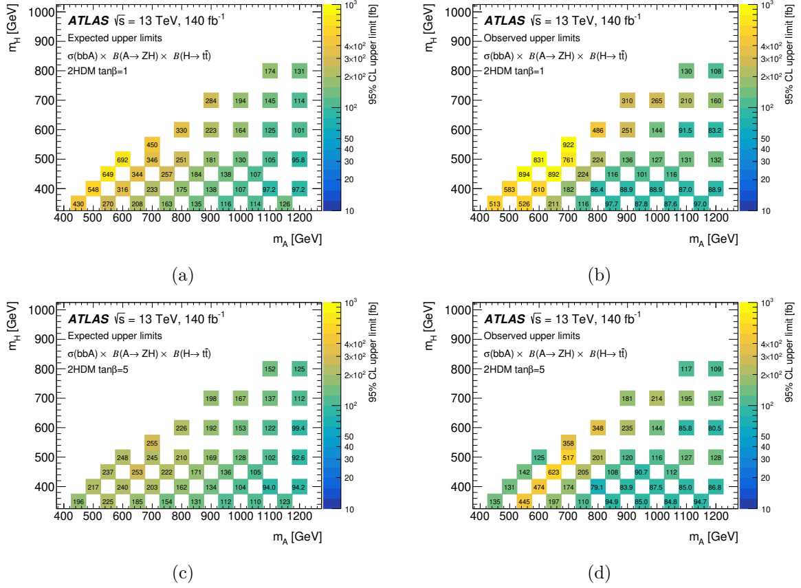
Figure 10. Expected and observed upper limits at 95% CL on \sigma(bb\bar{A}) \times B(A \rightarrow ZH) \times B(H \rightarrow t\bar{t}) . The limits are shown for \tan\beta = 1 (a,b) and \tan\beta = 5 (c,d). The \tan\beta value is relevant only for the choice of A boson width.
