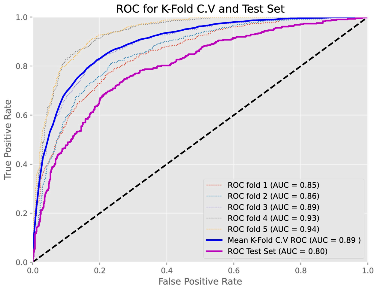
Fig 2. Training/Test set comparison. Training and Test AUCs and ROC curves for XGB + MICE + SMOTE model using Core variables upon predicting At-Risk MASH.
