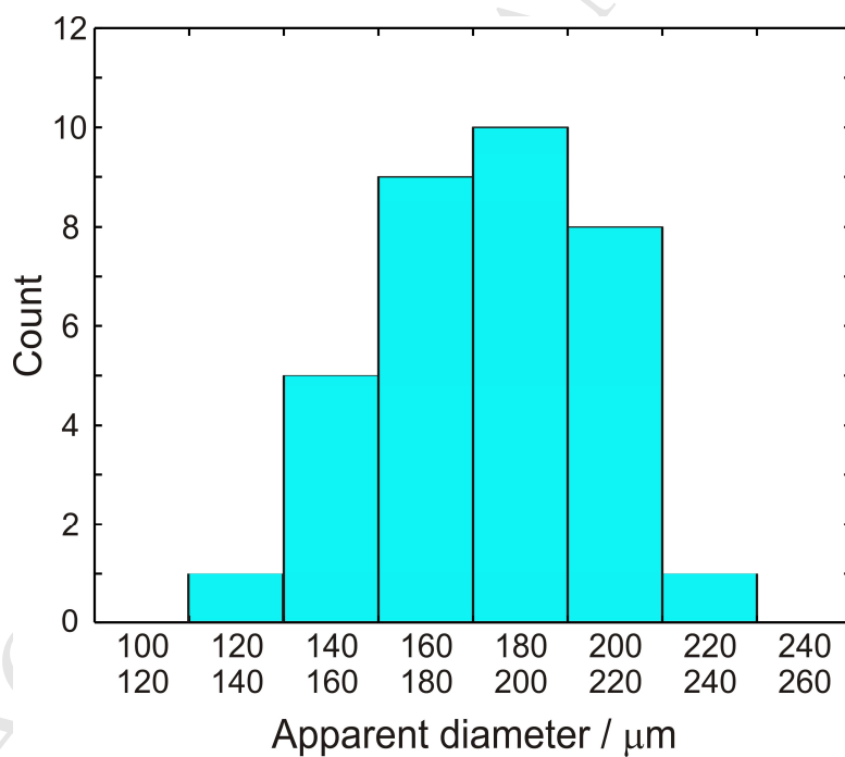
Figure 7 – Apparent size distribution of the particles surveyed during the course of the investigation (upper and lower limit if size range in \mu\text{m} ).
