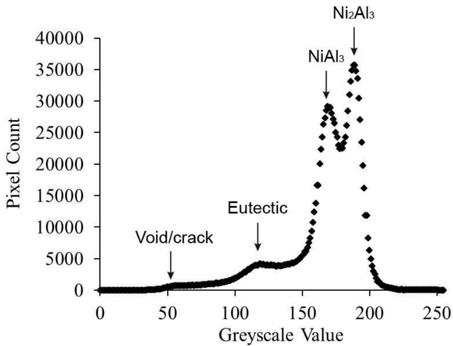
Figure 5 – Grey scale density distribution for the particle shown in Figure 3 .
