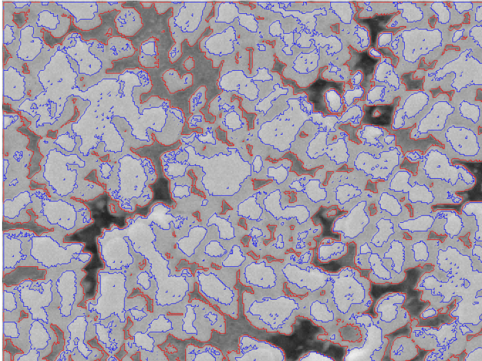
Figure 6 – A zoomed-in portion of Figure 3 showing the use of the ImageJ contour plotting add-on to establish density ranges for each phase.
