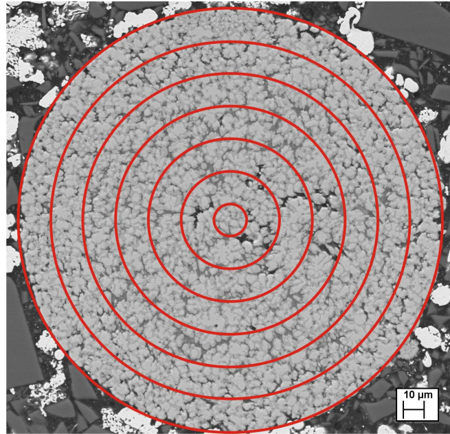
Figure 3 – Electron backscatter image of a particle showing density variations due to different phases. Contrast outside the particle circumference is due to electrically conductive mounting compound. Also shown are the positions of the annuli used in the quantitative analysis discussed in Section 2.3.
