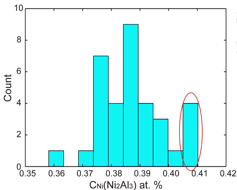
Figure 12 – Ni content of the \text{Ni}_2\text{Al}_3 phase based on a particle by particle mass balance calculation for the data shown in Figure 9 . The Ni-rich particles circled are the same group as circled in Figure 9a .
