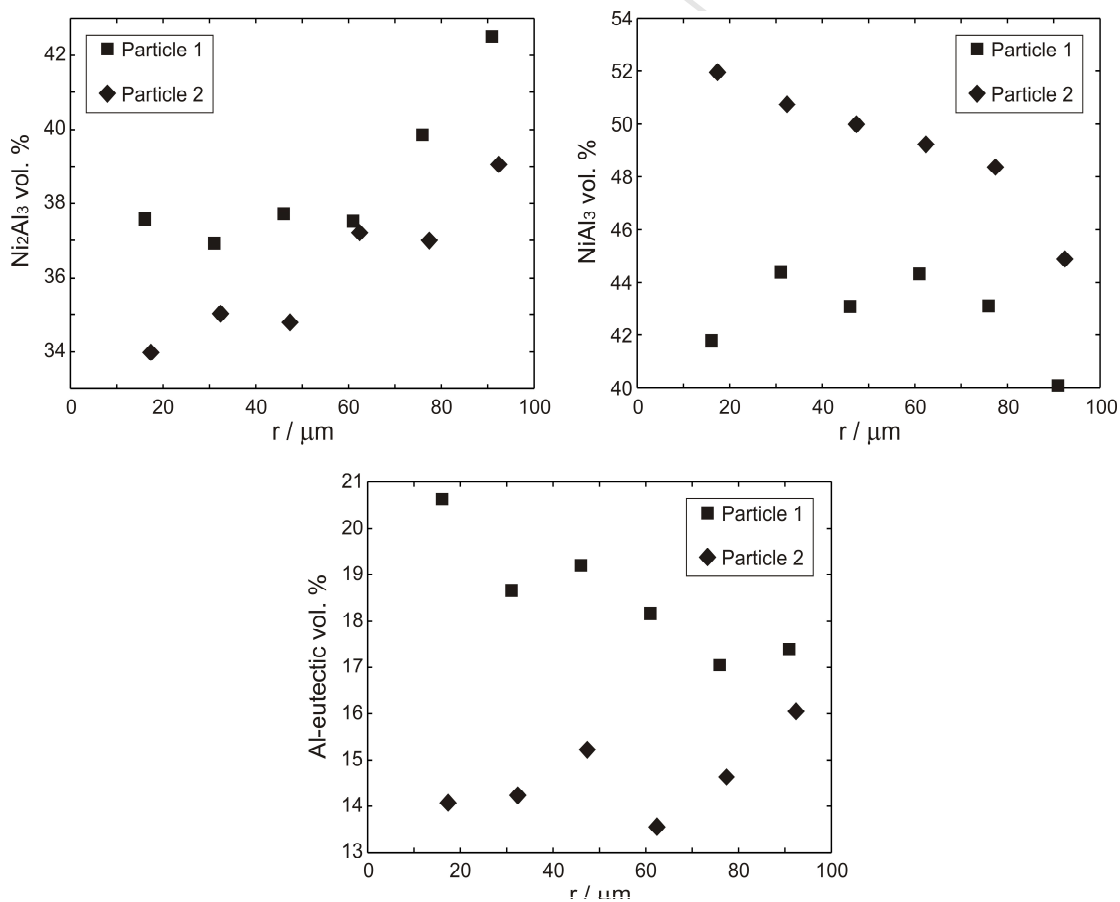
Figure 8 – Phase composition as a function of radial co-ordinate r for two typical particles analysed.
