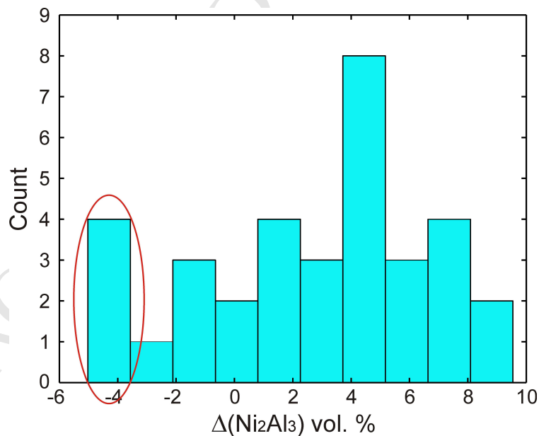
Figure 10 – Difference in \text{Ni}_2\text{Al}_3 content between the centre and outer most annulus for the particles investigated in this study (positive difference indicates more \text{Ni}_2\text{Al}_3 retained in the outer most annulus of the particle). The particles circled are the same group as circled in Figure 9a .
