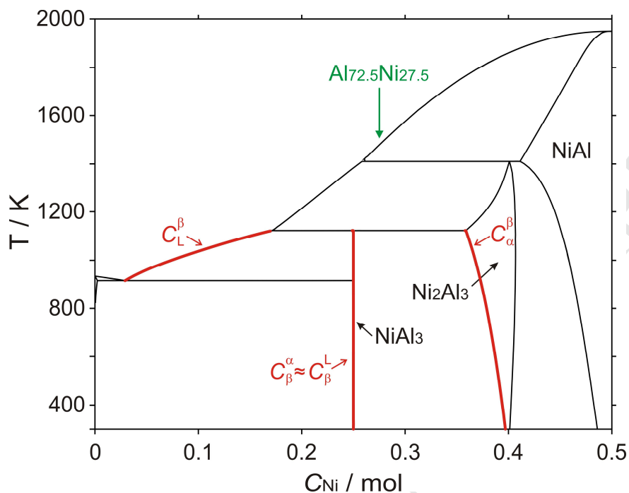
Figure 1 –Al-rich portion of the Al-Ni phase diagram showing the main phases present in Raney type Ni catalyst precursor alloys (Ni 2 Al 3 , NiAl 3 and Al-NiAl 3 eutectic), together with the 27.5 at.% starting composition of the liquid which forms the basis for this study. C_{\beta}^{\alpha} etc. refer to the terms in Equ. (1), which describes the rate at which the solid-solid peritectic transformation occurs, in this case with reference to the Ni 2 Al 3 + L → NiAl 3 peritectic (see below).
