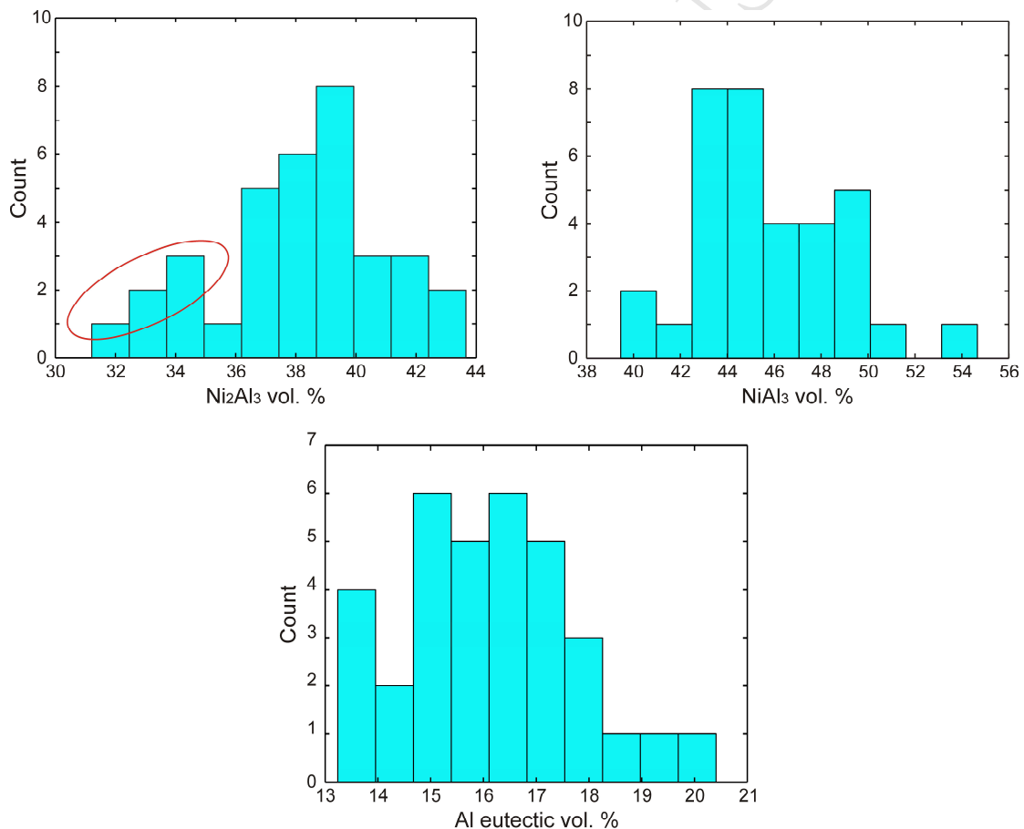
Figure 9 – Average phase composition for the particles investigated in this study. The possibly bimodal distribution for \text{Ni}_2\text{Al}_3 content is highlighted.
