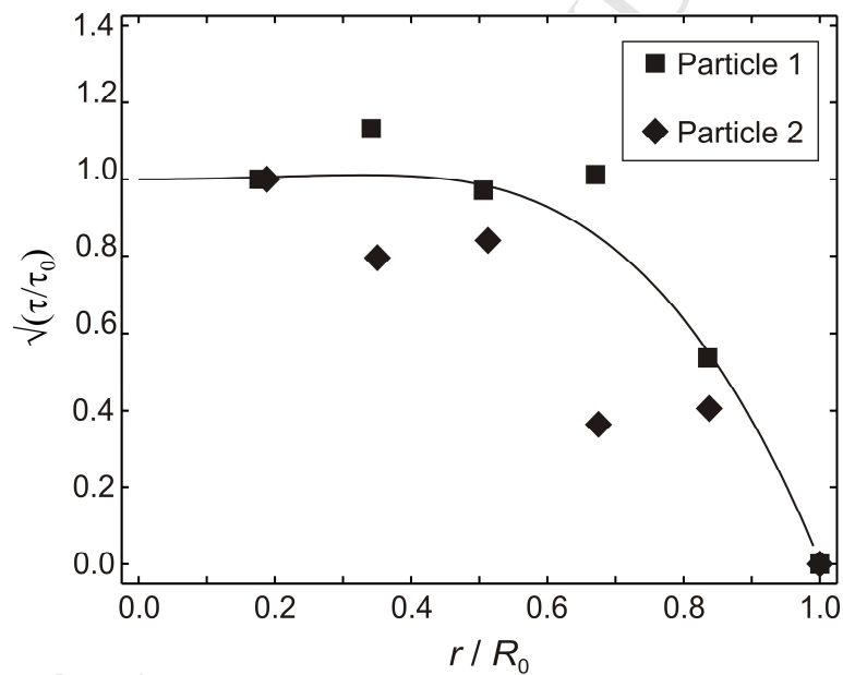
Figure 11 – Results of the cooling rate calculation (solid line) showing the relative difference in time available for the \text{Ni}_2\text{Al}_3 + \text{L} \rightarrow \text{NiAl}_3 peritectic transformation as a function of the radial co-ordinate r . Also shown the amount of \text{Ni}_2\text{Al}_3 transformed normalised by the peritectic for the two particles shown in Figure 8 (normalised to 0 at the surface and 1 at the centre of the particle).
