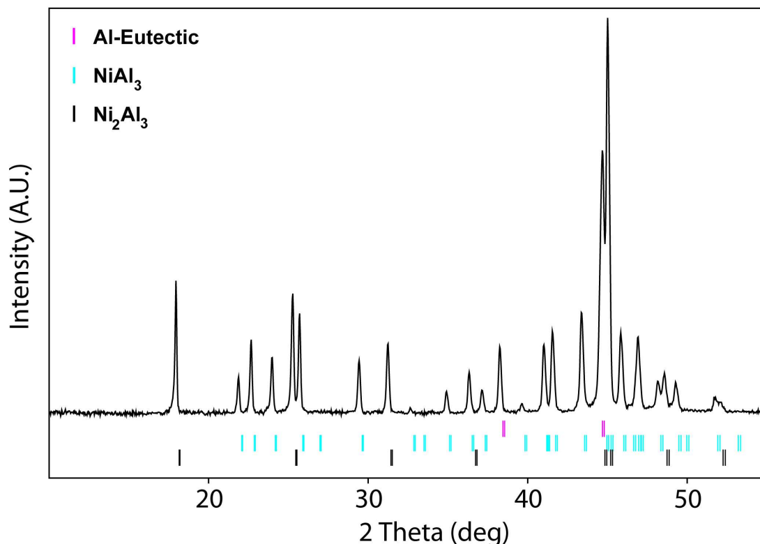
Figure 2 – XRD trace for the Al-27.5 at.% Ni alloy studied here, showing the presence of \text{Ni}_2\text{Al}_3 , \text{NiAl}_3 and \alpha\text{-Al} only.
