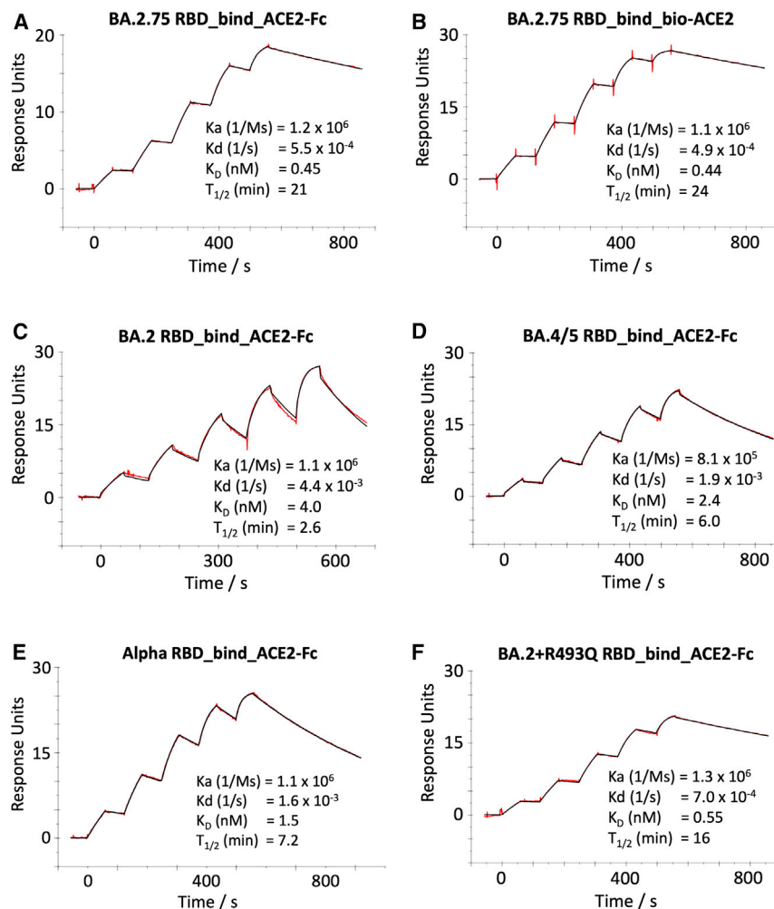
Figure 3. ACE2/RBD affinity
