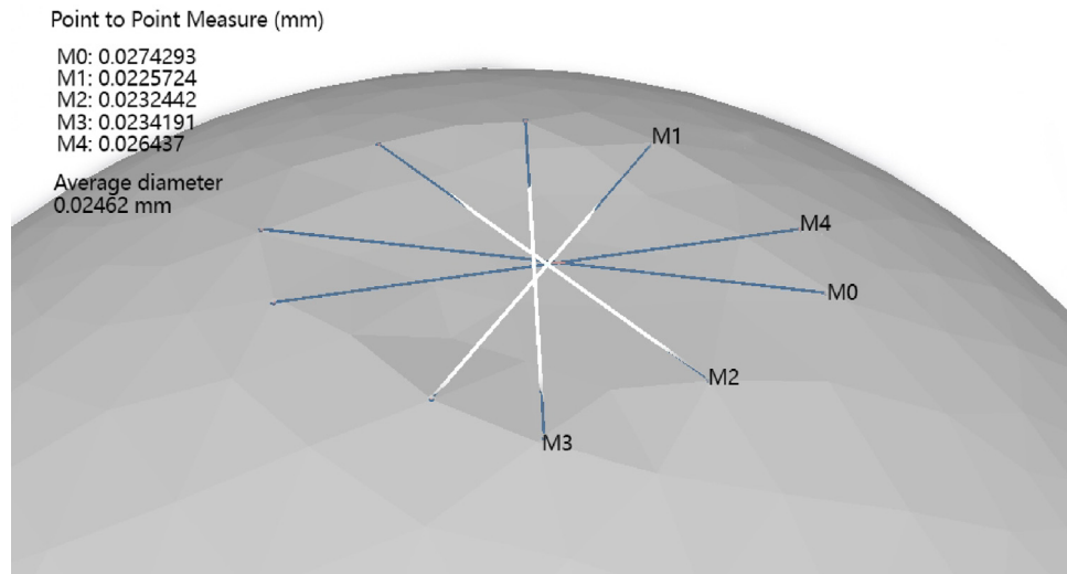
Fig. 13. Simulated dent formation and its dimensions (mm) for the 130 \mu\text{m} particle with 18 m/s relative velocity.
