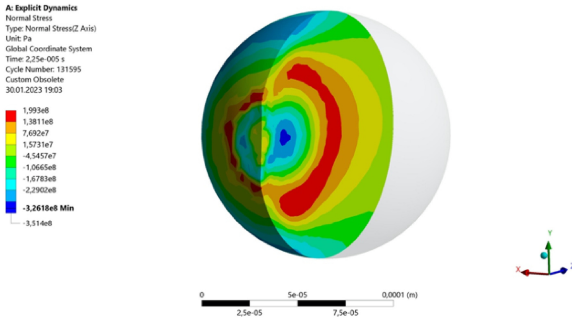
Fig. 12. Stress values obtained after simulation of 130 \mu\text{m} particle collision in ANSYS Explicit considering an 18 m/s relative velocity.
