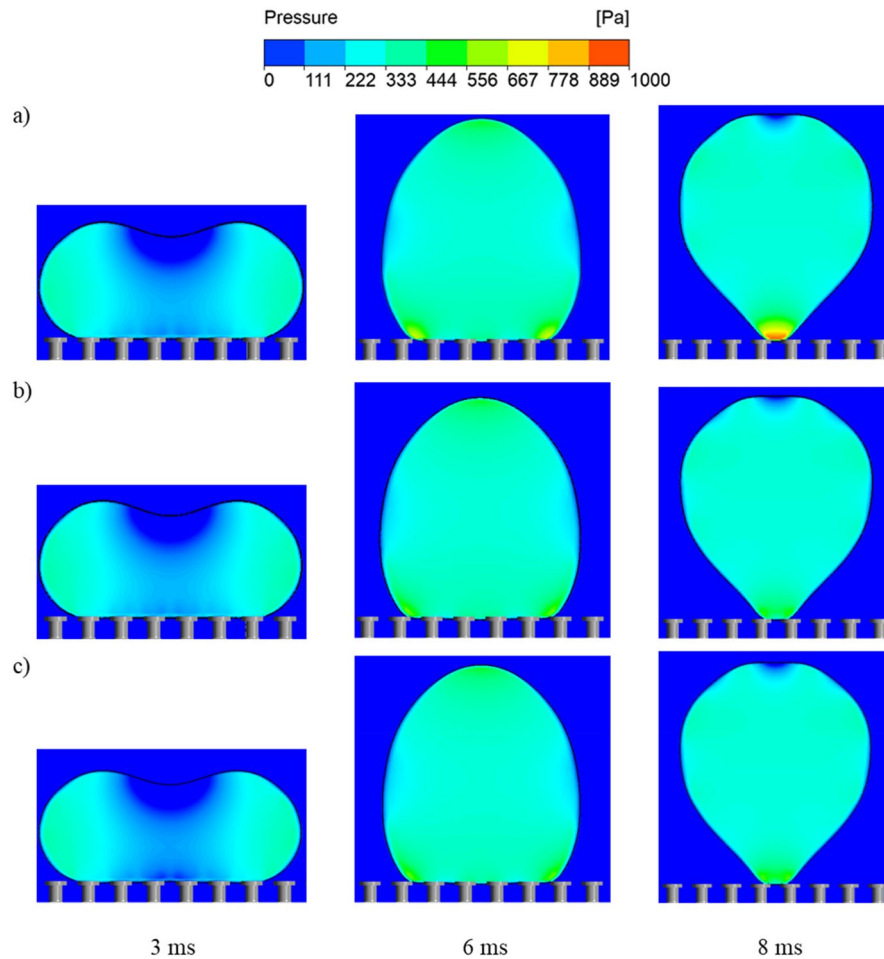
Figure 10. Pressure contours of impacting droplets on doubly re-entrant pillars at multiple time steps for various overhang thicknesses: (a) t_o = 5 \mu\text{m} , (b) t_o = 10 \mu\text{m} , (c) t_o = 15 \mu\text{m} .
