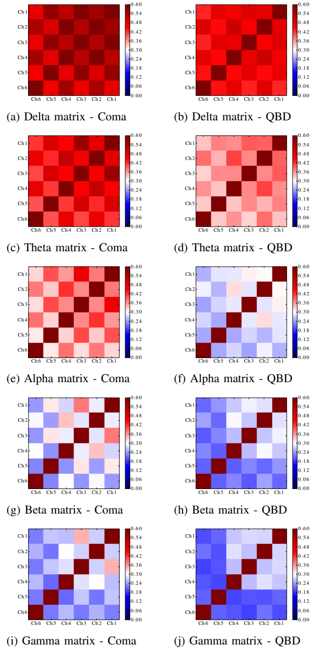
Fig. 2. Connectivity Matrix: Coma vs QBD with statistical analysis synchrony is important for understanding neuron integration, especially why it is particularly useful for the identification of coma and quasi-brain-death. Coma patients have the ability to shift individual chaotic actions to the ordered actions of a collective system. The “chaotic to ordered” process is reflected by phase synchrony, whereas brain death patients do not have the ability to conduct cognitive operations, therefore, phase synchrony for coma patients should be higher than that of QBD. The analysis results suggest the mean PSI for coma data, as shown in the matrices, is higher than in QBD.
