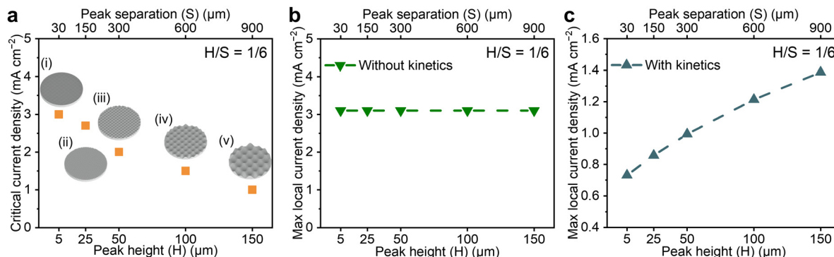
Fig. 2 Experimentally determined critical currents for dendrites and calculated maximum current densities for egg-box contoured surfaces with the same ratio of peak height ( H ) to separation ( S ). (a) Experimentally determined critical currents for all five constant H/S ratio surfaces (orange squares), the 3D simulated surfaces for each are also shown in grey (i) H5S30 (ii) H25S150 (iii) H50S300 (iv) H100S600 (v) H150S900. (b) Calculated maximum (max) local current density without including Li deposition kinetics for all five constant H/S ratio surfaces for 1 \text{ mA cm}^{-2} geometrical current density. (c) Calculated maximum (max) local current density including Li deposition kinetics for all five constant H/S ratio surfaces for 1 \text{ mA cm}^{-2} geometrical current density.
