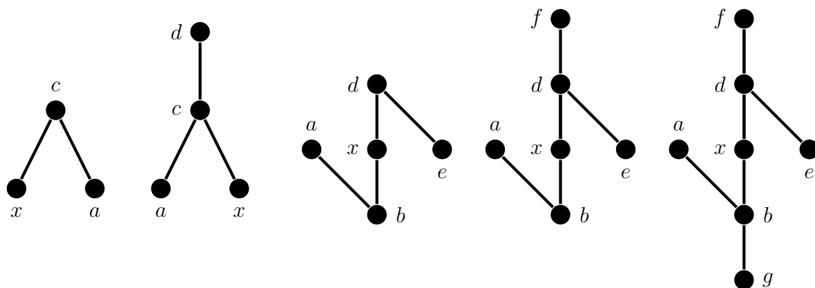
Figure 3: The Hasse diagrams of the \wedge , Y^d , S , S^+ , and S^{++} posets.
