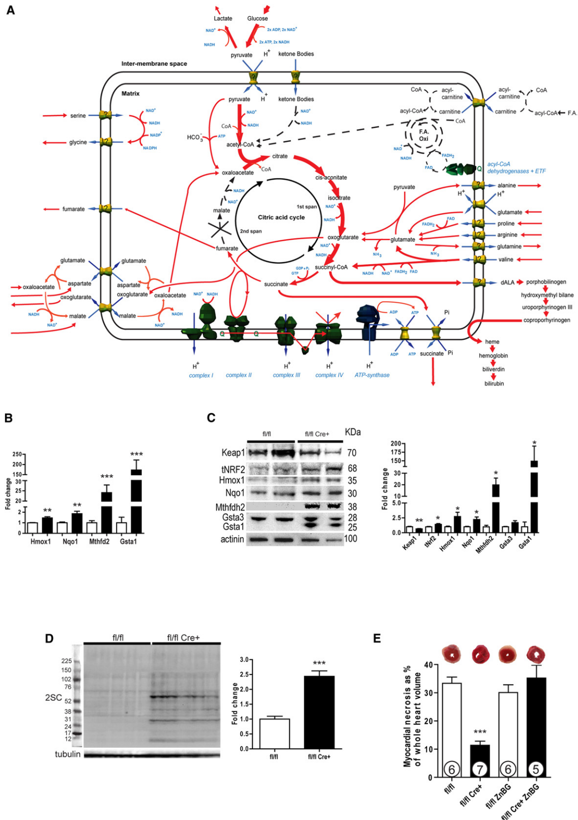
Figure 4. Fh1 Deficiency Confers Cardioprotection through Both Increasing Carbon Flux and Upregulating Heme Oxygenase 1 by Nrf2
