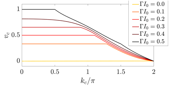
FIG. 17. Critical velocity as calculated from the Bogoliubov dispersion within a region -k_c \leq k \leq k_c . For k_c = 2\pi or larger, v_c = 0 for all stable nonlinearities, indicating that the system is not superfluid. However, for lower values of k_c , a nonvanishing v_c \neq 0 is found in the presence of a finite nonlinearity, indicating that “superfluid-like” behavior may be observed for sufficiently wide defects.
