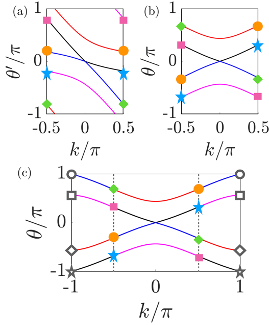
FIG. 5. (a) Bogoliubov quasi-energy dispersion (18) for \Gamma_0 = 0.2 in the moving frame. The continuous connection of the bands across the first Brillouin zone boundaries with the unusual boundary conditions of this Method (see also Fig. 3) are indicated by the symbols; bands with (j, \eta) = (-1, -1), (-1, 1), (1, -1), (1, 1) are colored in pink, blue, black, and red, respectively (as ordered from the bottom to the top at k = 0 ). (b) The dispersion of (a) Galilean transformed back into the laboratory frame via \theta = \theta' + k . (c) The extended zone scheme between -\pi \leq k < \pi constructed from (b) (with the first Brillouin zone marked by vertical gray dotted lines). This is fully equivalent to the Bogoliubov dispersion obtained via Method 2, shown in Fig. 4, with the colors of the curves now also showing the symmetry condition on the states. With respect to this larger momentum range, the dispersion is periodic and has normal boundary conditions (as indicated by open gray symbols).
