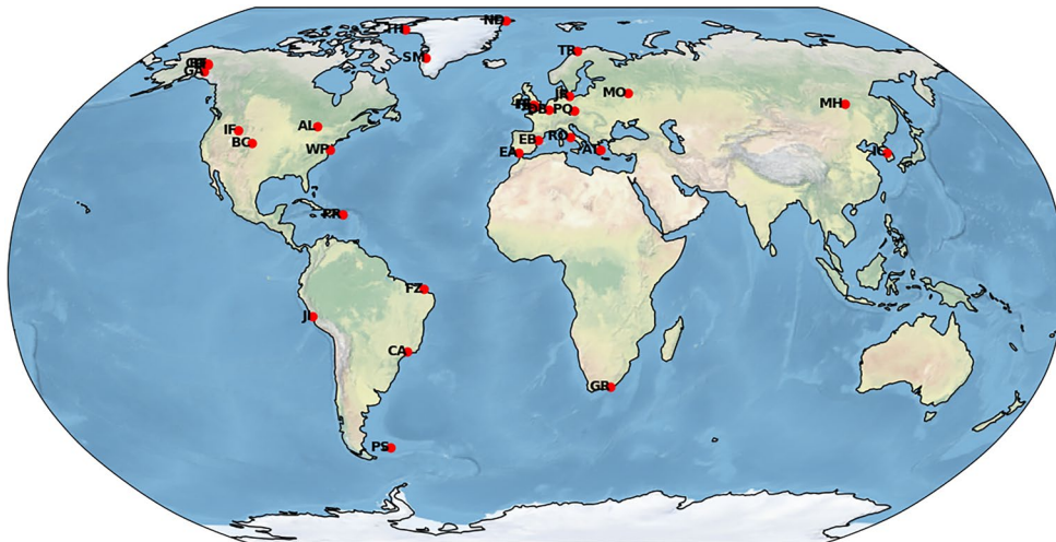
Figure A1. Ionosonde stations used to train the ML classifier.
