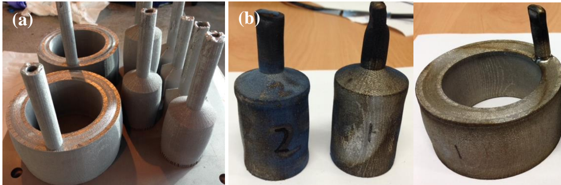
Fig. 3 Photographs showing several tooling designs (a) before and (b) after HIPing
