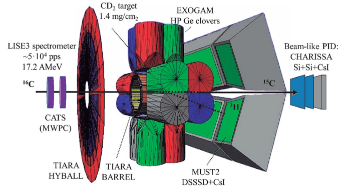
Fig. 1. Schematic view of the experimental set-up.
