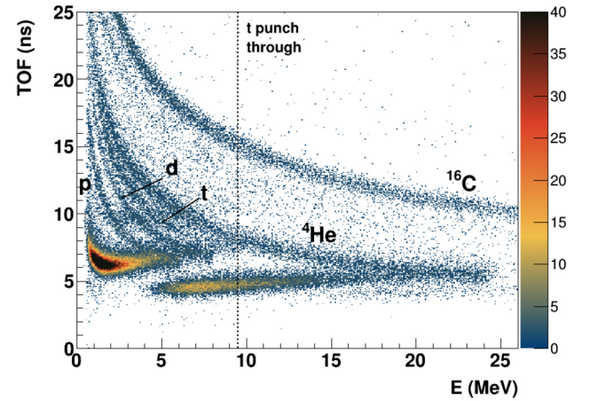
Fig. 2. Identification matrix: Time-Of-Flight (TOF) in ns between MUST2 and the first beam tracking detector versus the energy in MeV measured in the first layer of the MUST2 telescope. The dashed line shows the triton punch-through.
