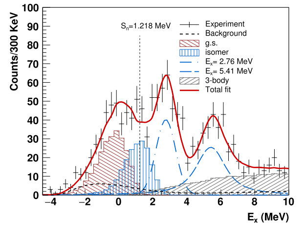
Fig. 4. Experimental excitation energy spectrum for ^{15}\text{C} obtained in the reaction ^{16}\text{C}(d, t)^{15}\text{C} for the angular range 3^\circ – 15^\circ in the center of mass. Bound states are represented by histograms obtained from simulations (see text) while dash-dotted curves correspond to the unbound states. The light grey filled histogram shows the contribution from the three-body final state ( ^{14}\text{C}+n+t ) and the dashed line that from the background from neighbouring masses. The solid-red curve is the total fit to the spectrum.
