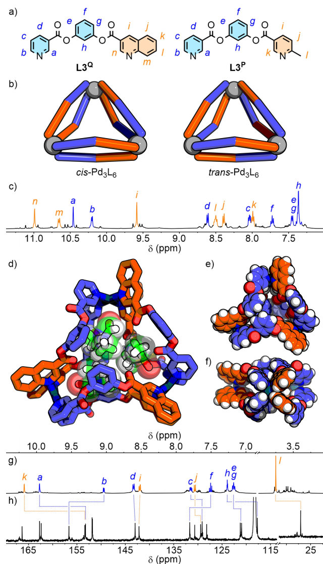
Figure 5. a) Ligands L3 Q and L3 P ; b) schematic representations of \text{Pd}_3\text{L}_6 ‘double-walled’ triangle isomers with all- cis and all- trans donor arrangements; c) ^1\text{H} NMR spectrum (500 MHz, d_6 -DMSO) of C3 Q ; SCXRD structure of cis - C3 Q showing d) cis - C3 Q in \text{DMF}_2\text{DMSO} , and space filling representation e) from the top, and f) from the side; g) ^1\text{H} NMR spectrum (500 MHz, \text{CD}_3\text{CN} ) and h) ^{13}\text{C} NMR spectrum (126 MHz, \text{CD}_3\text{CN} ) of C3 P .
