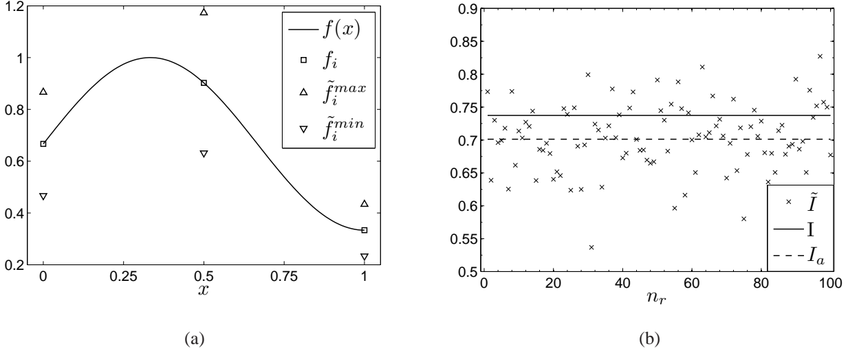
Figure 1: Evaluation of pest abundance from noisy data. (a) An example of the pest population density function f(x) . Three equidistant traps are installed over the unit interval to measure the density f(x) . The density value \tilde{f}_i , i = 1, 2, 3 measured at the position x_i of the trap lies within the range (10) with probability P(z) as defined by (11). The lower and upper limits of this range are denoted \tilde{f}_i^{\min} and \tilde{f}_i^{\max} respectively. The measurement tolerance has been set as \nu_m = 0.3 and we have fixed z = 3 . (b) The distribution of the estimate \tilde{I} of pest abundance computed from the measured data \tilde{f}_i on a grid of N = 3 traps. Each realisation is presented as a skewed cross in the figure, where n_r = 100 realisations of the estimate \tilde{I} are shown. The values \tilde{I} are compared with the exact value I of the pest abundance (solid line) and the estimate I_a computed from the exact data f_i (dashed line).
