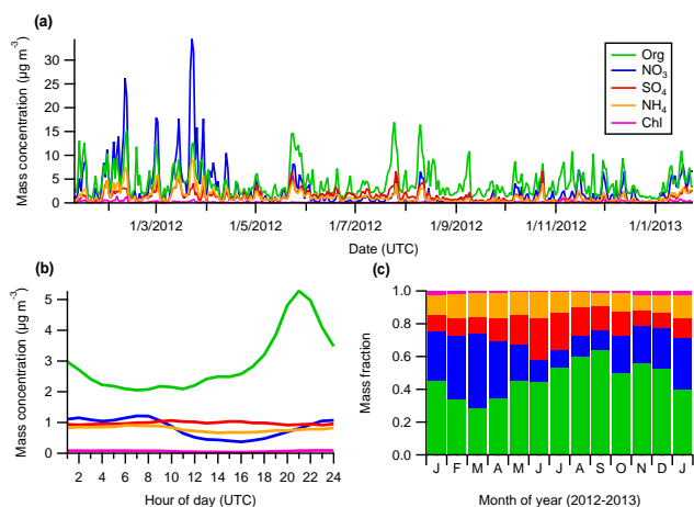
Figure 1. (a) Daily averaged time series of all NR-PM 1 species. (b) Median diurnal profiles of all NR-PM 1 species. (c) Average monthly fractional contribution of all species to total NR-PM 1 . The months are grouped as seasons: January 2012, February, December, and January 2013 are in winter; March, April, and May are in spring; June, July, and August are in summer; September, October, and November are in autumn.
