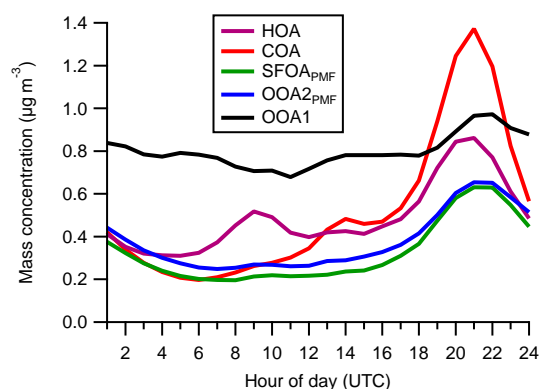
Figure 3. Median diurnal profiles for each of the five PMF factors. Note that these data do not include a period from the summer (see Sect. 4.1).
