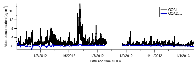
Figure 4. Time series of OOA1 and OOA2 mod , where OOA2 mod is the daily average.
