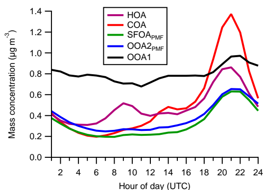
Figure 3. Median diurnal profiles for each of the five PMF factors. Note that these data do not include a period from the summer (see Sect. 4.1).
