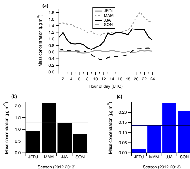
Figure 6. (a) OOA1 seasonal median diurnal profiles. (b) Average seasonal concentration of OOA1, with the annual average denoted by the thick horizontal line. (c) Average seasonal concentration of OOA2 mod , with the annual average concentration denoted by the thick horizontal line, both estimated in Sect. 4.4. Note that these data do not include the summer period (see Sect. 4.1).
