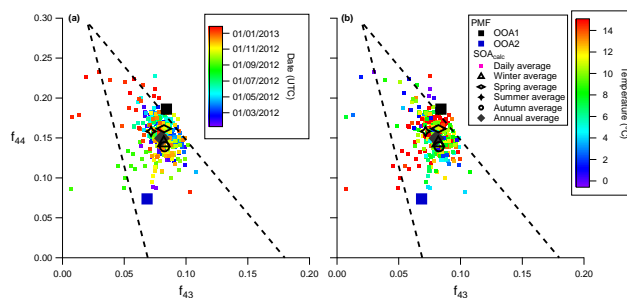
Figure 7. Daily averaged SOA within f_{44} vs. f_{43} space coloured by time (a) and temperature (b), where f_{44} and f_{43} refer to m/z 44:SOA calc and m/z 43:SOA calc respectively. See text for more details. Daily averaged temperatures ranged from -0.5 to 26 °C, although they are only coloured here up to a maximum of 15 °C for clarity. Average annual and seasonal f_{44}/f_{43} values for SOA are denoted in the legend. OOA1 and OOA2 PMF factors are also plotted. The outline of the triangle as defined by Ng et al. (2010) is shown by the dashed black lines. Note that the organic data do not include the summer period (see Sect. 4.1).
