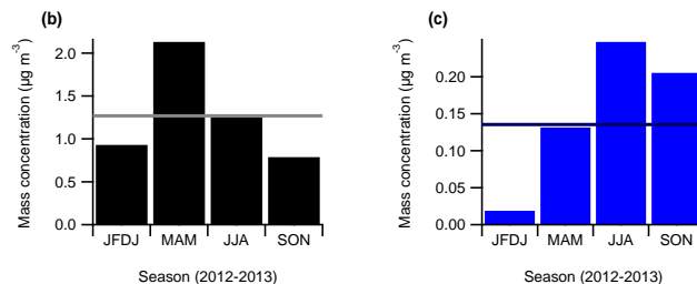
Figure 6. (a) OOA1 seasonal median diurnal profiles. (b) Average seasonal concentration of OOA1, with the annual average denoted by the thick horizontal line. (c) Average seasonal concentration of OOA2 mod , with the annual average concentration denoted by the thick horizontal line, both estimated in Sect. 4.4. Note that these data do not include the summer period (see Sect. 4.1).
