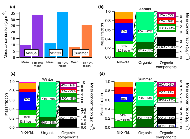
Figure 8. (a) Mean concentrations of the full calendar year (2012–2013), winter, and summer months. The average concentration of the top 10th percentile for the year as well as the top 10th percentile in the winter and summer are also shown. (b) Average fractional contributions of all species to the top 10th percentile for the year, with an expansion of the organic fraction into each of its primary and secondary components. (c) Average fractional contributions of all species to the top 10th percentile in the winter, with an expansion of the organic fraction into each of its primary and secondary components. (d) Average fractional contributions of all species to the top 10th percentile in the summer, with an expansion of the organic fraction into each of its primary and secondary components. In all figures, SFOA and OOA2 refer to SFOA mod and OOA2 mod respectively. Note that the PMF data (middle and right bars) do not include the summer period as detailed in Sect. 4.1 as well as Sects. 4.1 and 4.2 in the Supplement.
