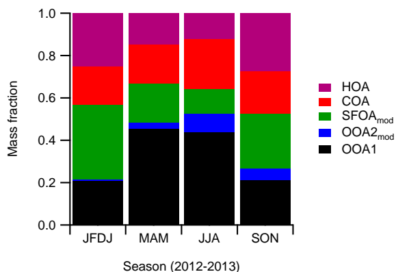
Figure 5. Seasonal fractional contributions of the PMF factors to total OA mass, with revised masses (see Sect. 4.4). As discussed in Sect. 4.1, a period from the summer is not included in these data.
