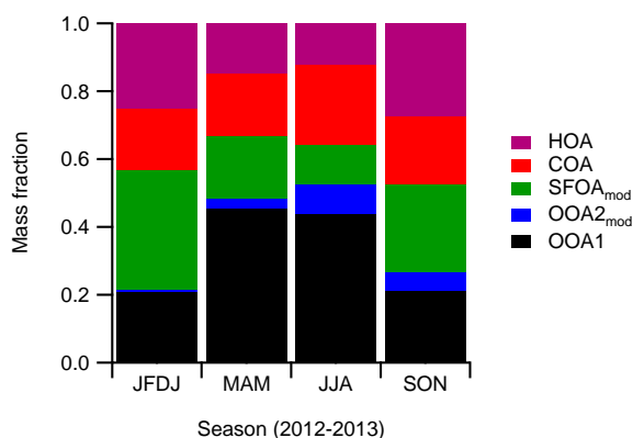
Figure 5. Seasonal fractional contributions of the PMF factors to total OA mass, with revised masses (see Sect. 4.4). As discussed in Sect. 4.1, a period from the summer is not included in these data.
