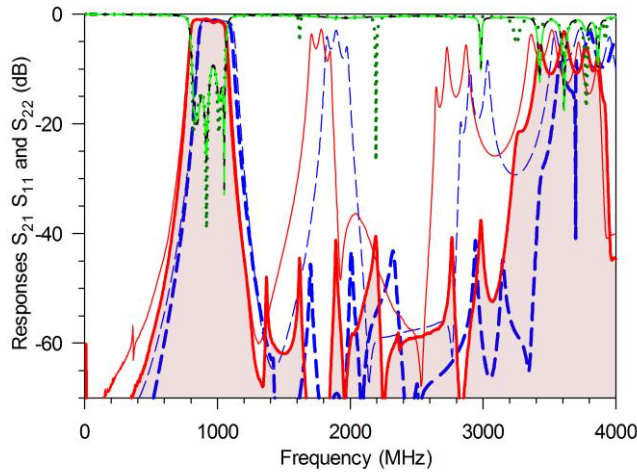
Fig. 12. 8% bandwidth filter response (see fig. 10 for legend).
