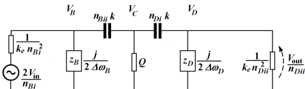
Fig. 8. Filter equivalent circuit, with the center resonator resonating.
