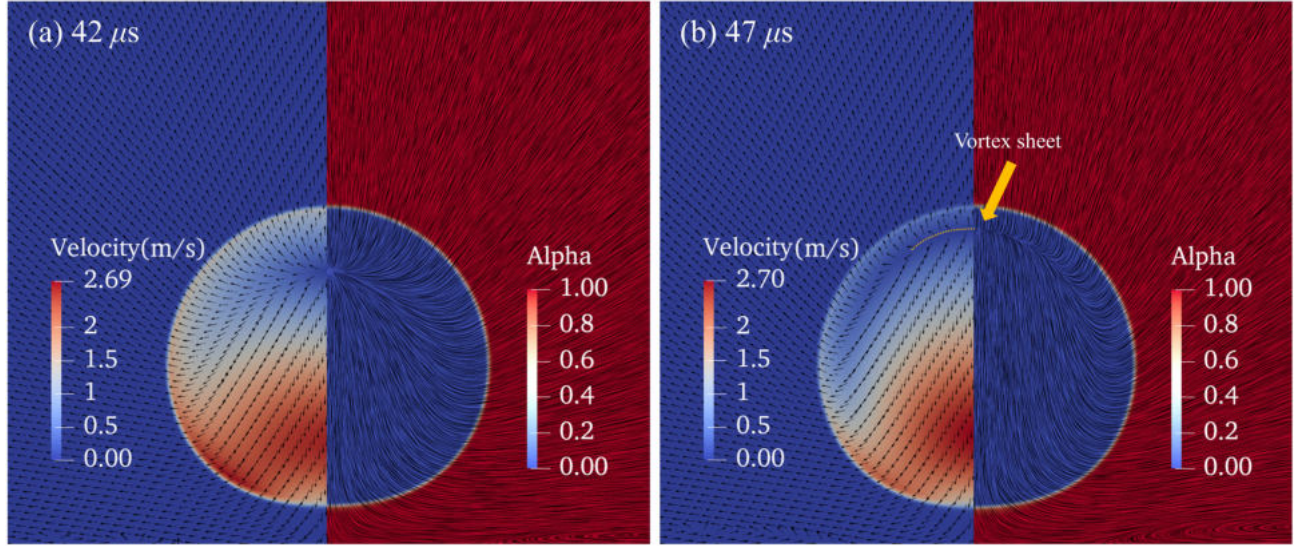
FIG. 14. Velocity vectors (left in each figure), velocity contours (left in each figure), and streamlines (right in each figure) at (a) 42 \mu s and (b) 47 \mu s showing the formation of the vortex sheet generated from the bubble collapse near a rigid boundary for the case of Re = 75 in figure 13. (Recall that the simulations are axisymmetric when visualizing the 3D form of the vortex sheet).
