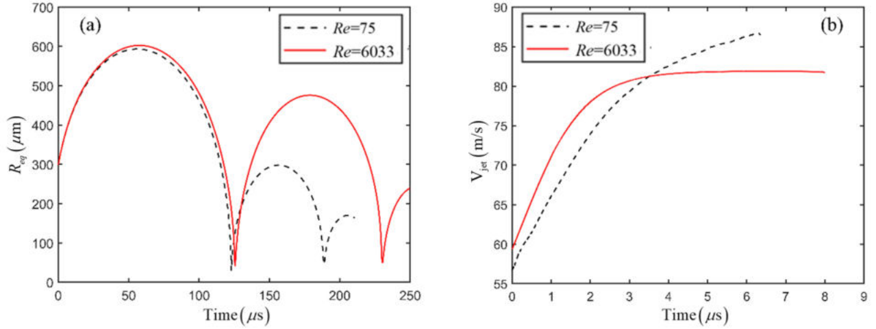
FIG. 18. Numerical results for Re = 75, 6033 ( \mu_l = 0.08, 0.001 \text{ Pa} \cdot \text{s} , respectively): (a) histories of the equivalent bubble radius R_{eq} and (b) the jet velocity V_{jet} with the time counted from the jet starting ( t = 114 \mu\text{s} for Re = 6033 and t = 116 \mu\text{s} for Re = 75 ). The remaining parameters are the same as in figure 4.
