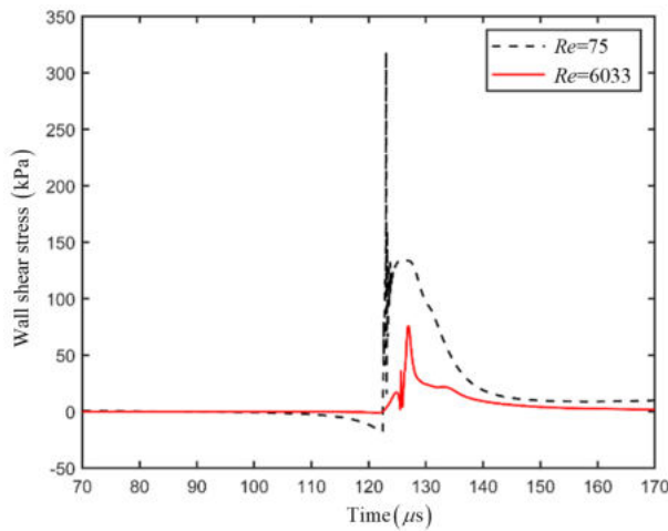
FIG. 23. The time histories of the shear stress at a point on the rigid boundary, at 180 \mu\text{m} from the axis of symmetry, for Re = 75, 6033 ( \mu_l = 0.08, 0.001 \text{ Pa} \cdot \text{s} , respectively). Other parameters are the same as in figure 4.
