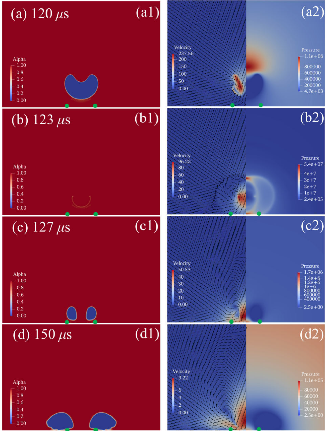
FIG. 24. Bubble shapes (frames (a1)-(d1)) and flow fields (frames (a2)-(d2)) including velocity vectors (left in frames (a2)-(d2)), velocity contours (left in frames (a2)-(d2)) and pressure contours (right in frames (a2)-(d2)) at (a) 120 \mu s , (b) 123 \mu s , (c) 127 \mu s , and (d) 150 \mu s during bubble collapse and rebound for the case of Re = 75 in figure 13.
