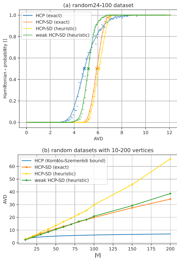
Fig. 5. Comparison of Hamiltonicity bounds.
