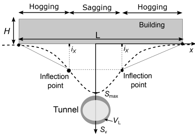
Fig. 3. Description of the settlement trough, building geometry and sagging and hogging zones.
