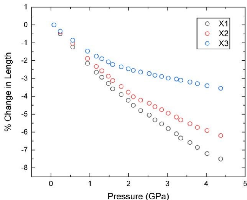
Figure 4. Percentage changes in lengths of principal axes with increasing pressure according to the powder neutron diffraction data
