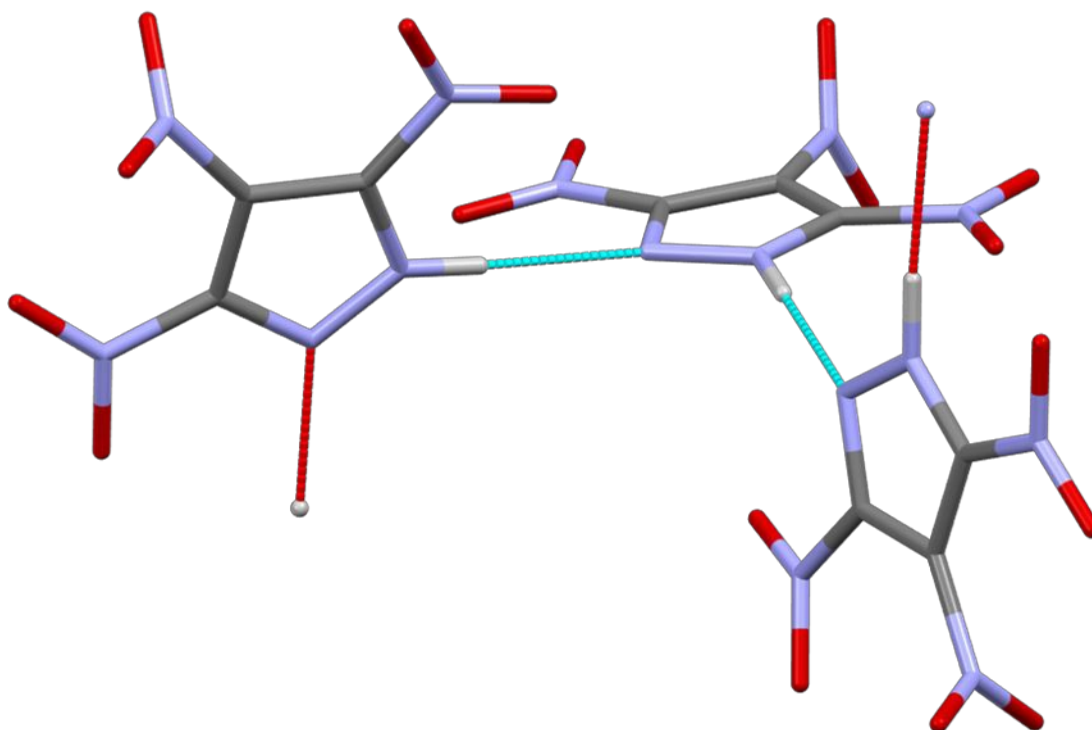
Figure 1. Arrangement of 3,4,5-TNP molecules in the crystal structure of Form I. Intermolecular hydrogen bonding interactions are shown by the blue and red dashed lines. Nitrogen atoms shown as blue, carbon as grey, oxygen as red and hydrogen as white.
