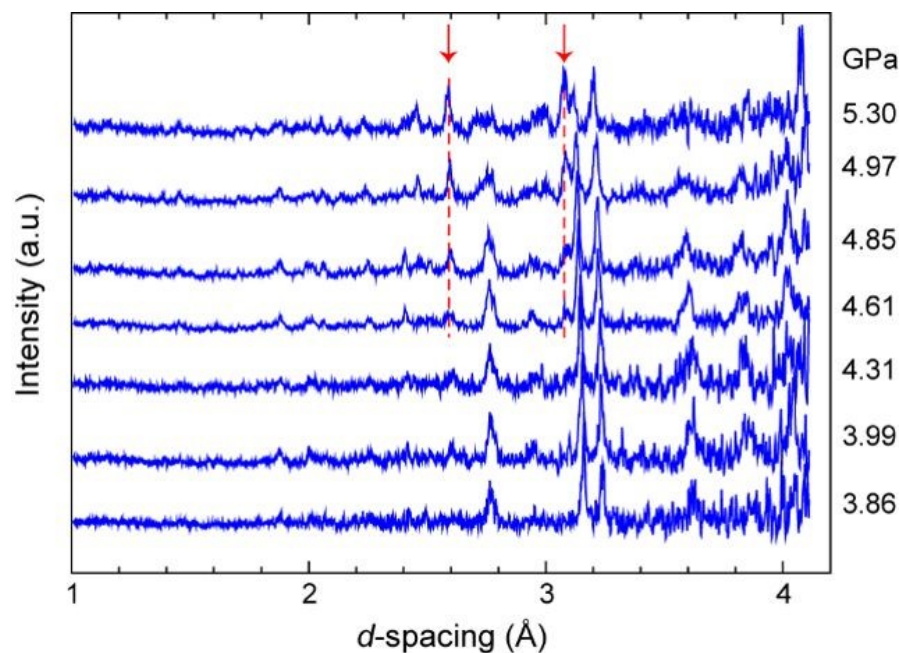
Figure 5. Sequence of powder neutron diffraction patterns obtained for 3,4,5-TNP from the second loading using WC anvils over the pressure range 3.86 – 5.30 GPa. Red dashed lines indicate the appearance or disappearance of peaks associated with the sluggish phase transition.
