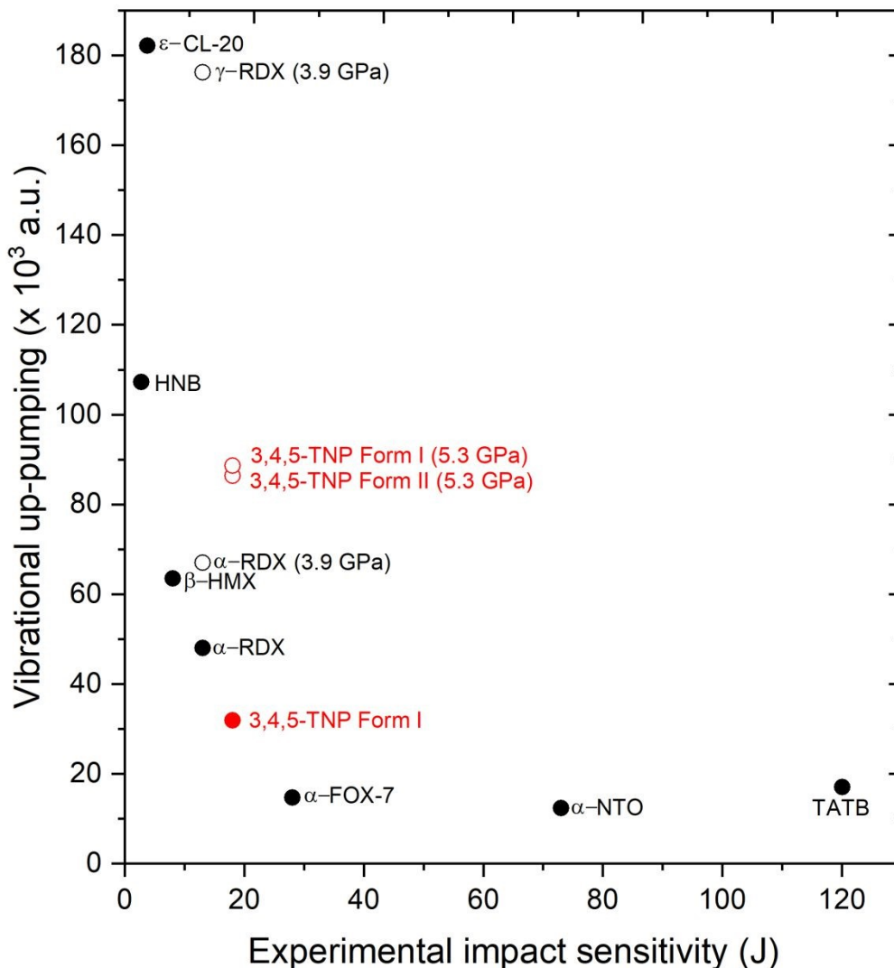
Figure 10. Vibrational up-pumped densities versus experimental IS values for a range of EMs alongside predictions for Forms I and II of 3,4,5-TNP, shown in red. Filled symbols correspond to experimentally measured data points, unfilled to predicted values only. Experimental value selected for TATB is based on an estimate from reference 56.
