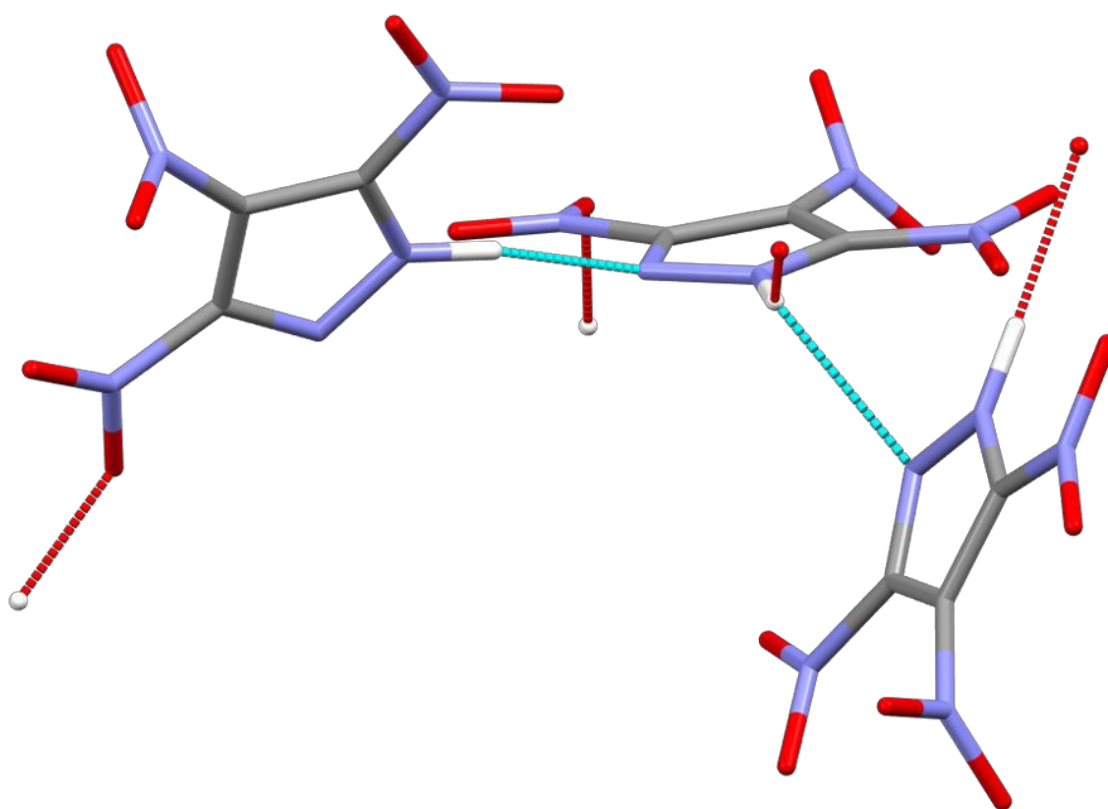
Figure 8. Arrangement of 3,4,5-TNP molecules in the crystal structure of Form II, illustrating bifurcated hydrogen bonding interactions around the central molecule. Nitrogen atoms shown as blue, carbon as grey, oxygen as red and hydrogen as white.
