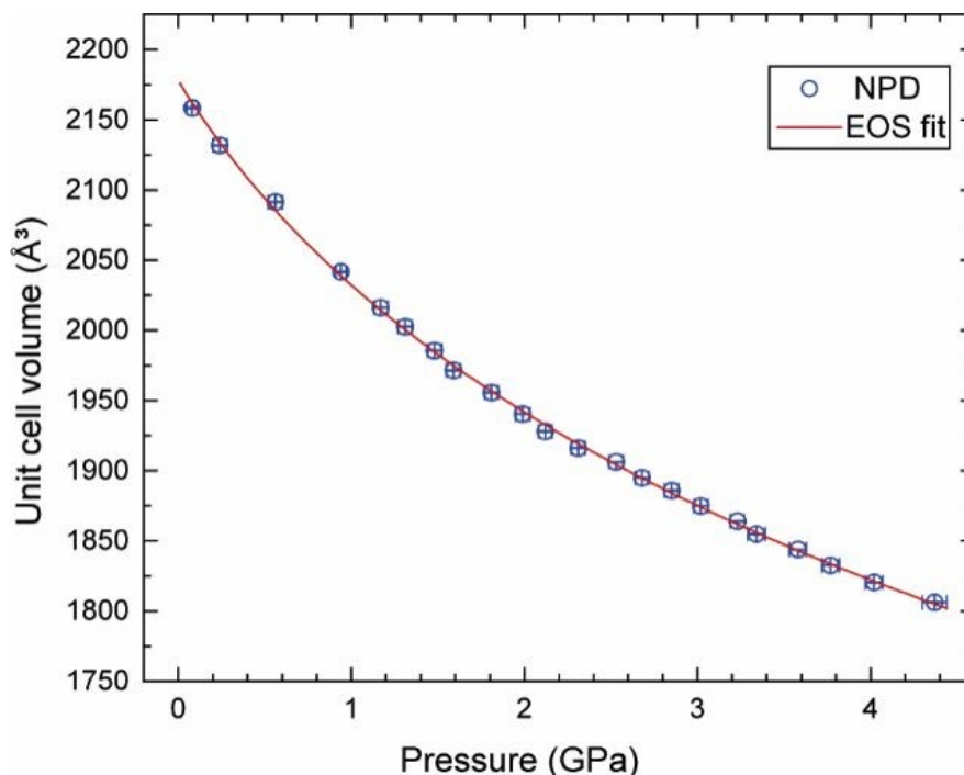
Figure 3. Variation of unit-cell volume as a function of pressure determined from neutron powder diffraction data for 3,4,5 TNP (open blue circles) and the EoS fit from P–V data (solid red line). Error bars are shown, but are smaller than the symbols.
