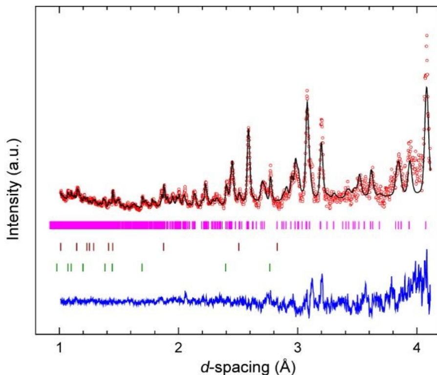
Figure 6. Rietveld refinement of the powder neutron diffraction pattern of 3,4,5-TNP recorded at 5.3 GPa. Red circles are the neutron diffraction data; the black line represents the fit to the data based on the structure of Form II determined by X-ray diffraction, including scattering contributions from Pb and WC; the blue line is the difference plot, I(\text{obs}) - I(\text{calc}) . Tick marks represent positions of Bragg peaks from 3,4,5-TNP (magenta), Pb (green), and WC (red).
