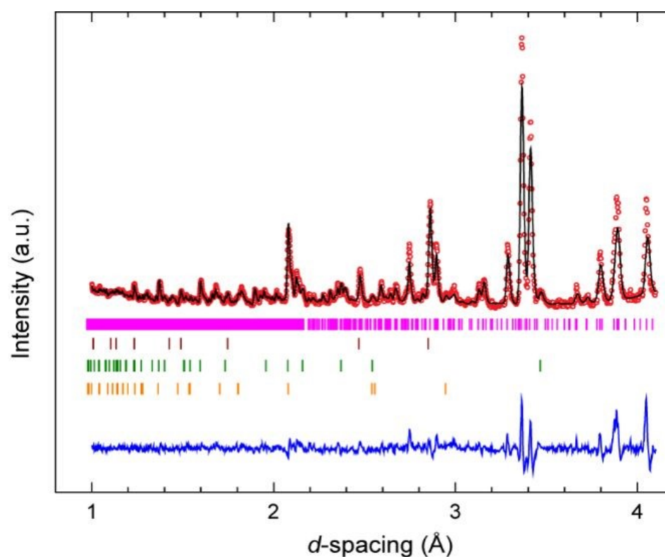
Figure 2. Rietveld refinement of neutron powder diffraction pattern of 3,4,5-TNP at 0.08(3) GPa (space group P2_1/c ); red dots are experimental (observed) data, solid black line is the calculated profile from the refinements, while the bottom blue line shows the residual intensities I(\text{obs})-I(\text{calc}) . Simulated Bragg reflections for each phase are shown as vertical tick marks: from top to bottom 3,4,5-TNP, Pb (the pressure calibrant), \text{Al}_2\text{O}_3 , and \text{ZrO}_2 (the anvil material).
