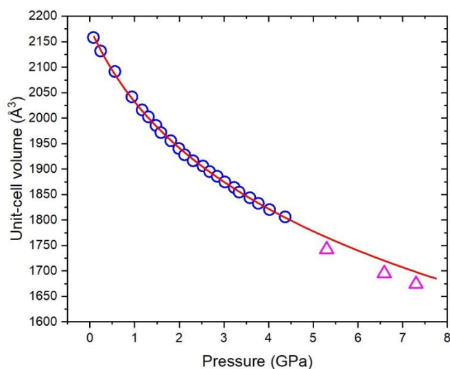
Figure 7. Variation of unit-cell volume as a function of pressure for Form I (open blue circles) obtained from neutron powder diffraction data; the EoS fit from P–V data (solid red line); and unit-cell volumes for Form II obtained from single crystal X-ray diffraction data
