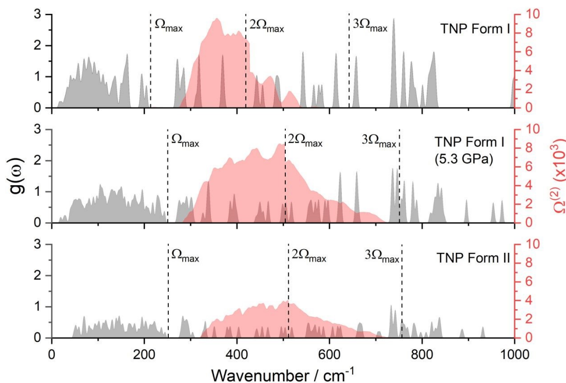
Figure 9. Vibrational g(\omega) plots (grey) for Form I at ambient pressure, Form I re-optimised at 5.3 GPa, and Form II at 5.3 GPa, alongside their corresponding \Omega^{(2)} envelopes (red).
