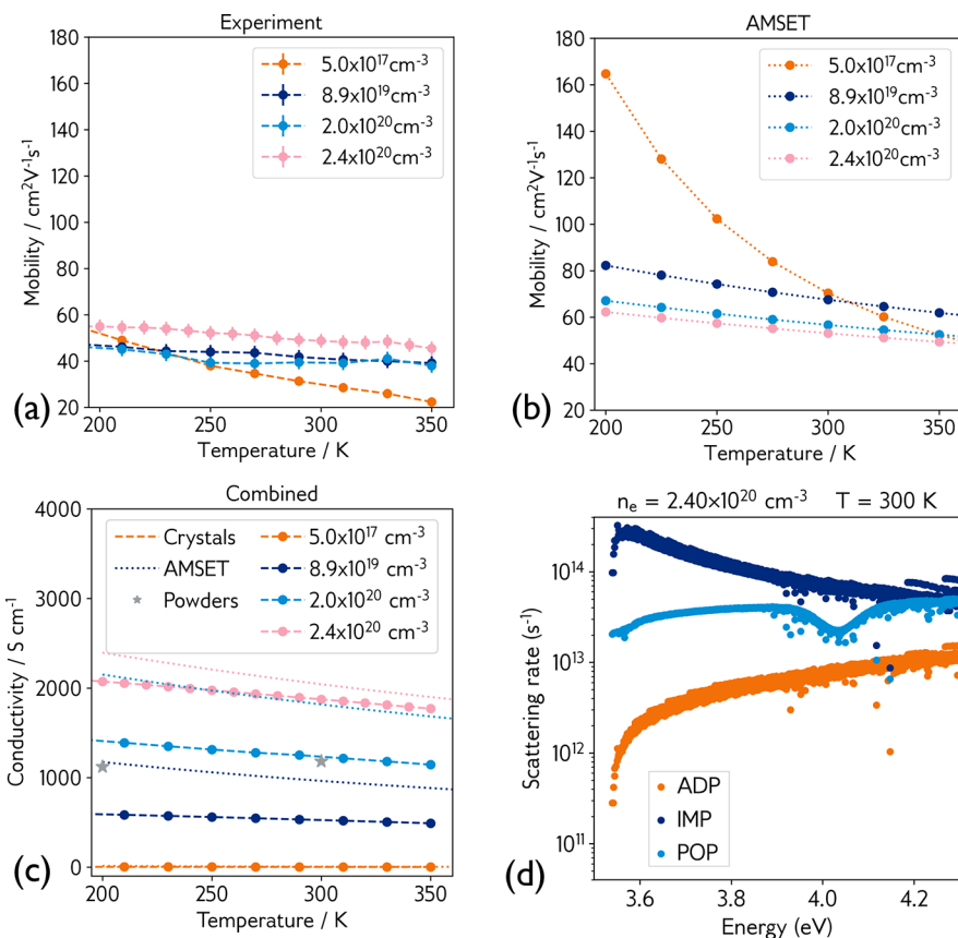
Figure 4. (a) Experimental mobility of undoped and Ga-doped single-crystal \text{ZnSb}_2\text{O}_6 . (b) Simulated (using AMSET) mobility of \text{ZnSb}_2\text{O}_6 at carrier concentrations measured from experiment. (c) Single-crystal and simulated conductivity over a range of carrier concentrations, with THz spectroscopy data for an 8% \text{Zn}_{1-x}\text{Ga}_x\text{Sb}_2\text{O}_6 solid solution plotted as gray stars. (d) Calculated room-temperature scattering rates at 2.4 \times 10^{20} \text{ cm}^{-3} . Abbreviations: ADP, acoustic deformation potential scattering; IMP, ionized impurity scattering; and POP, polar optical phonon scattering. Moving from low to high carrier concentrations causes a switch in dominant scattering from POP to IMP.
