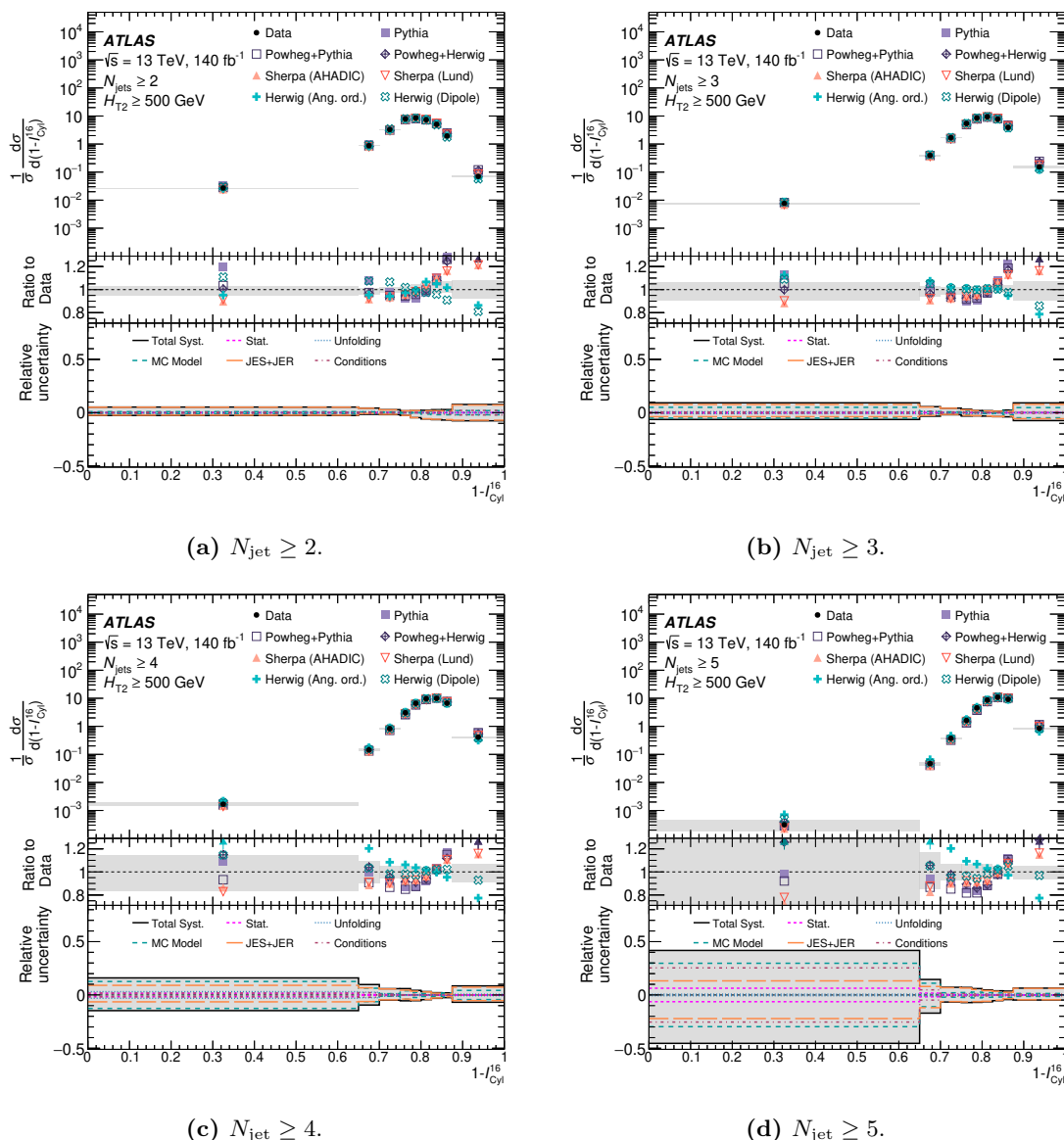
Figure 14. The shape-normalized \mathcal{I}_{Cyl}^{N=16} cross-section in data (closed circles), compared with predictions from several Monte Carlo generators. The distribution is presented for events with H_{T2} \geq 500 GeV, in several inclusive bins of N_{\text{jet}} . The middle panels display the ratios of different event generator predictions to the unfolded data. Event generator predictions are displayed as different marker styles. The grey band in the upper and middle panels indicates the total uncertainty of the measurement. If the ratio of a prediction to the unfolded data is outside the range of values displayed in the middle panels, an arrow is drawn at the edge of the panel as an indicator. The lower panels summarise the various sources of systematic uncertainty in the measurement. Systematic uncertainties are summarized in groups, with different line styles. The total uncertainty is shown as a solid black line.
