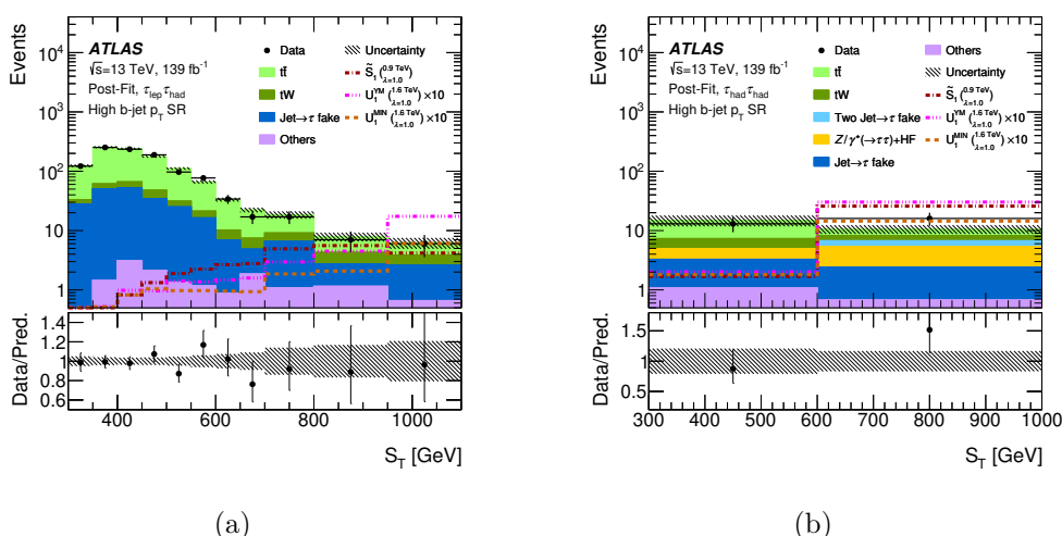
Figure 5. Post-fit distributions of the discriminating variable S_T in the high b -jet p_T signal region for the (a) \tau_{lep}\tau_{had} and (b) \tau_{had}\tau_{had} channels. The two channels are fit simultaneously considering the background-only hypothesis. The lower panels show the ratio of the data to the predictions, where the uncertainty band includes both statistical and systematic post-fit errors. Entries with values above the x -axis range are included in the last bin of each distribution. For illustrative purposes, the dotted lines show the expectation from three singly produced scalar and vector LQ signals.
