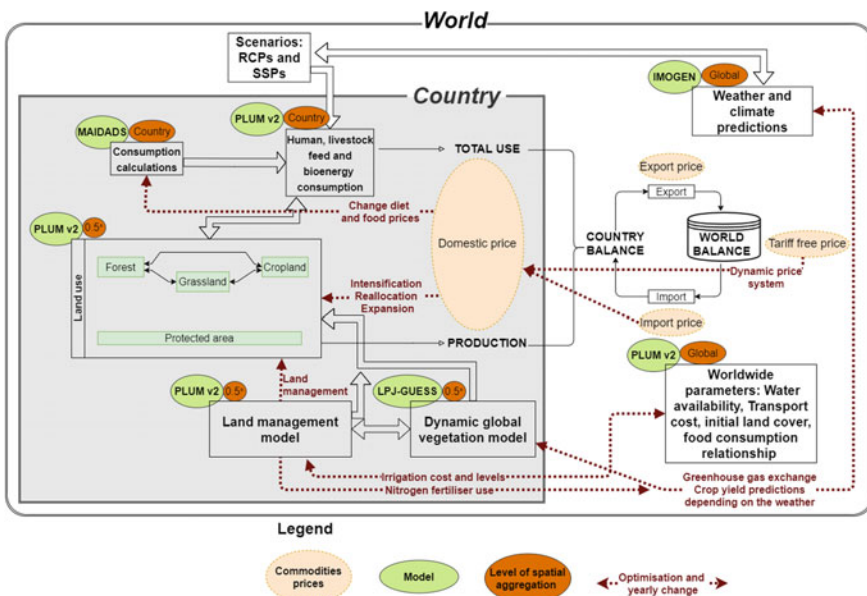
Fig. 16.1 LandSyMM structural overview. The focus of the schematic is on the cross-scale interactions between models (PLUMv2, LPJ-GUESS, IMOGEN, MAIDADS) and the embodied interactions between the country- and world-level calculations for each time step of the model. GDP: Gross Domestic Product; RCPs: representative concentration pathways; SSPs: shared socio-economic pathways
