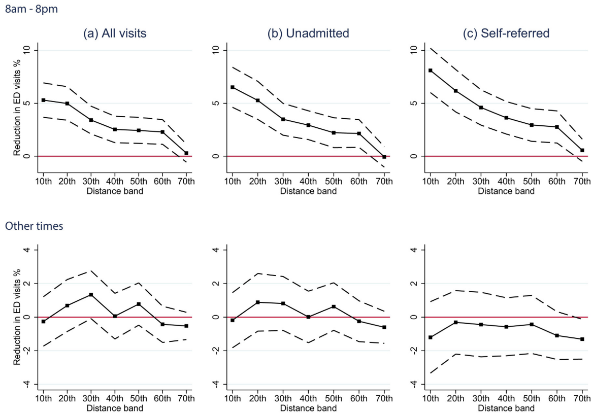
Fig. 7. Distance decay by ED visit type. Notes: Figure plots point estimates reported in Table A6 (black lines) and the bounds of the associated 95% confidence intervals.
