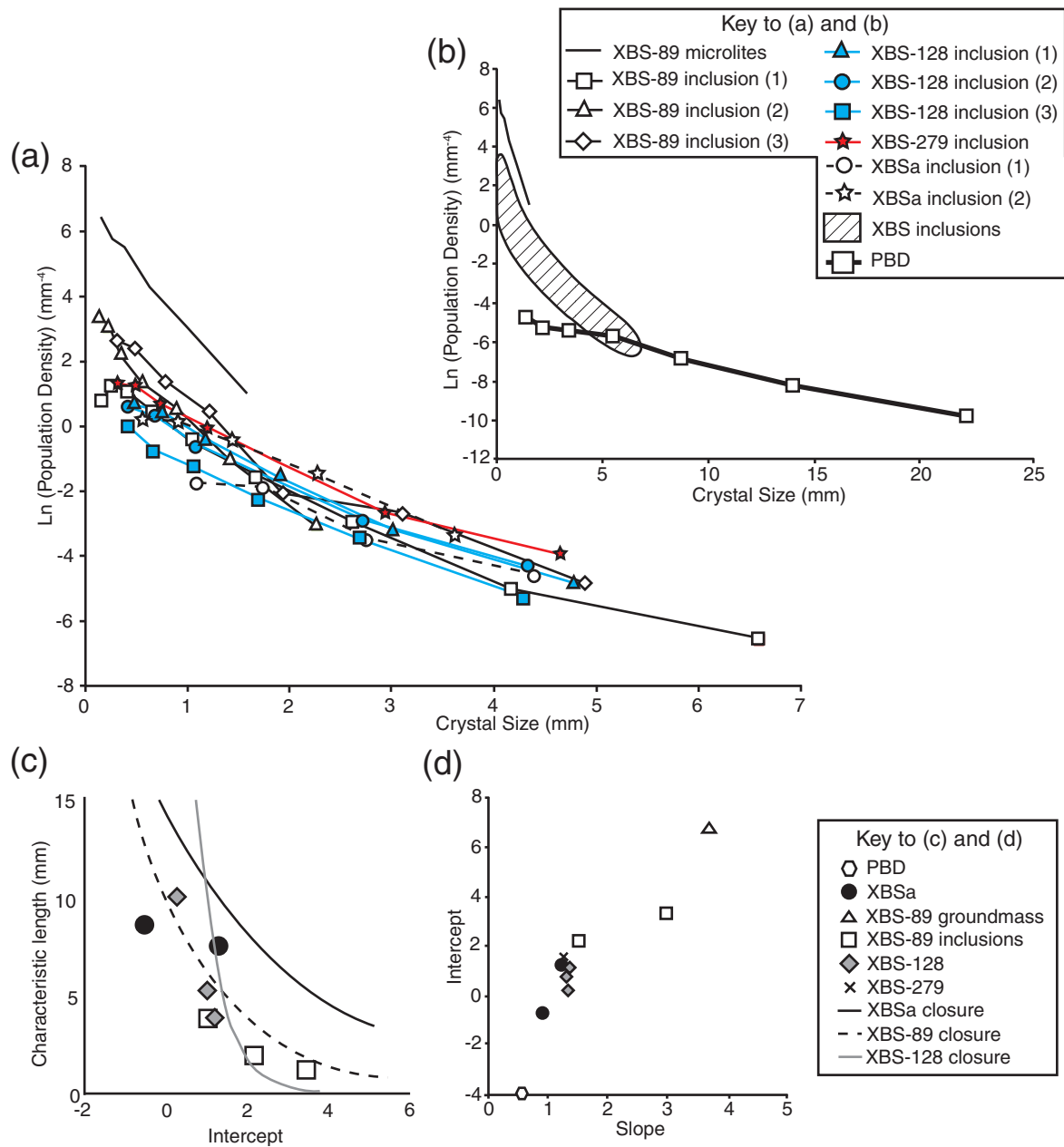
Fig. 10. CSD data for plagioclase crystals from (a) all samples except PBD and (b) all samples. (c) Characteristic length vs intercept plot for the inclusions, as more than one sample was measured for each, with the calculated closure limits. Closure limits, defined by the characteristic length for a volumetric abundance of 100% ( C_{100} ), are calculated after Higgins (2006b). (d) Intercept vs slope plot after Zeig & Marsh (2002).
