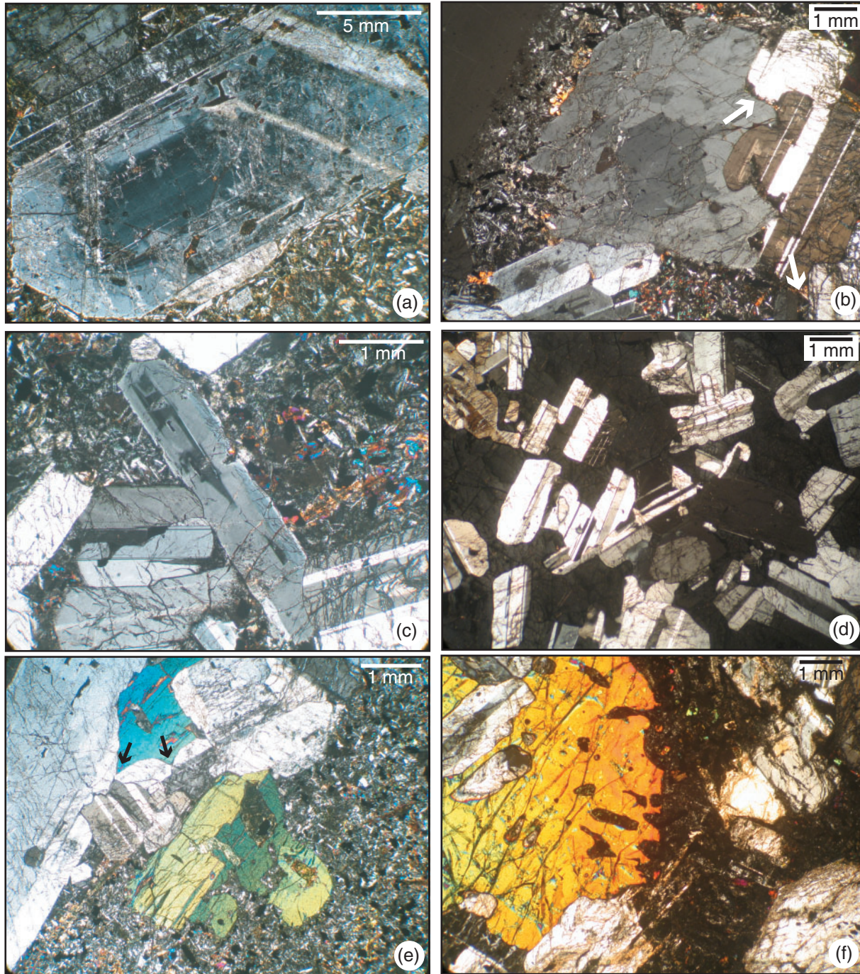
Fig. 6. Photomicrographs. (a) Chemical zoning of a cumulate plagioclase phenocryst within PBD. The randomly oriented plagioclase and clinopyroxene microlites at the bottom right should be noted. (b) Framework of tabular cumulus plagioclase within a gabbroic inclusion from XBSa. The pronounced chemical zoning of the middle plagioclase crystal and host magma groundmass along grain boundaries and at grain triple junctions should be noted (white arrows). (c) Complex resorption patterns within cumulus plagioclase crystals. The contact of the plagioclase with the host groundmass is irregular. (d) Clinopyroxene oikocryst (black) enclosing cumulus plagioclase. (e) Resorption texture exhibited in clinopyroxene within an inclusion of XBSa. Plagioclase–plagioclase–clinopyroxene triple junctions are also highlighted (black arrows). (f) Coarse clinopyroxene oikocryst in contact with the host groundmass and displaying evidence of resorption. All photomicrographs were taken with crossed polars.
