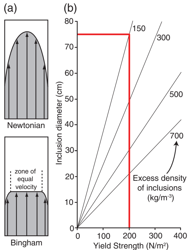
Fig. 12. (a) Schematic magma-velocity profiles for Newtonian and Bingham behaviour (after Correa-Gomes et al. , 2001). (b) The calculated minimum yield strength (bold line) required for a Bingham magma to entrain gabbro inclusions, derived from a crystal-mush, 75 cm in diameter (modified from Sparks et al. , 1977; Yoshinobu et al. , 2009).
