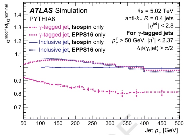
Fig. 8. PYTHIA 8-based evaluation of the impact of the isospin and nPDF effects for the two jet samples, shown as the ratio of the modified cross-section to the nominal one in pp collisions. The isospin (nPDF) effect for inclusive jets is shown as a solid (dotted) line, and for photon-tagged jets as dot-dashed (dashed) line.
