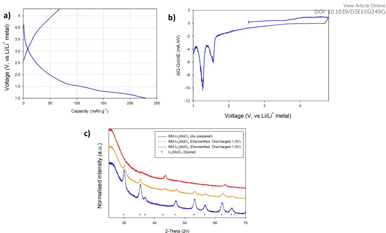
Figure 7: a) First cycle voltage profile for BM-Li 2 MoO 4 cycled in the region of 4.8 - 1.0 V at 10 mA g -1 ; b) associated dq/dv plot of the first charge/discharge cycle; c) PXRD of dismantled swagelok cells showing phases formed once discharged down to 1.5 and 1.0 V (Cu Kα).
