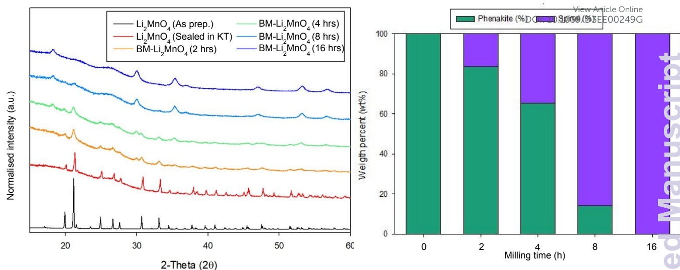
Figure 1: PXRD of samples prior to and after milling illustrating a transformation from phenakite to spinel structure (left), with the calculated phase fractions from Rietveld refinement (right). (Cu K\alpha ).
