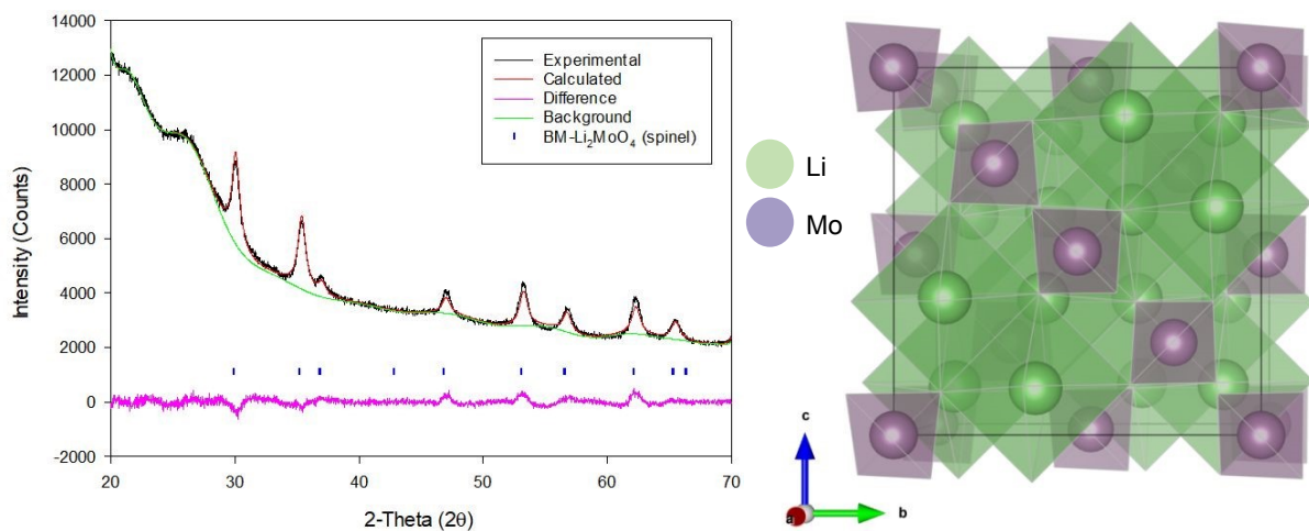
Figure 2: Observed, calculated and difference profiles for Rietveld refinement of \text{BM-Li}_2\text{MoO}_4 (16 h) (left) and an image of the spinel structure adopted by this phase (right). (Cu K\alpha ).
