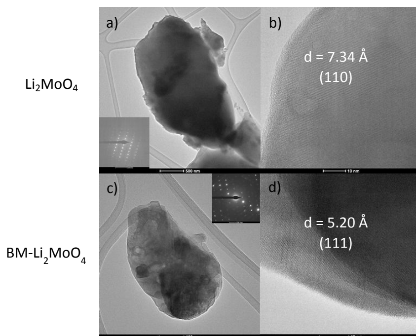
Figure 4: TEM images of pristine (a) and ball milled (c) \text{Li}_2\text{MoO}_4 particles, with inset images showing the SAD pattern recorded on the particles, and the respective HR-TEM images (b and d) clearly showing the lattice fringes. The observed interplanar distance from the fringes have been indexed.
