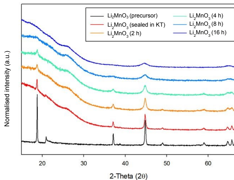
Figure 9: PXRD data for the timed milling study of \text{Li}_2\text{MnO}_3 (2 - 16 h at 450 rpm) showing a transition from a layered to DRS structure ( \text{Cu K}\alpha ).
