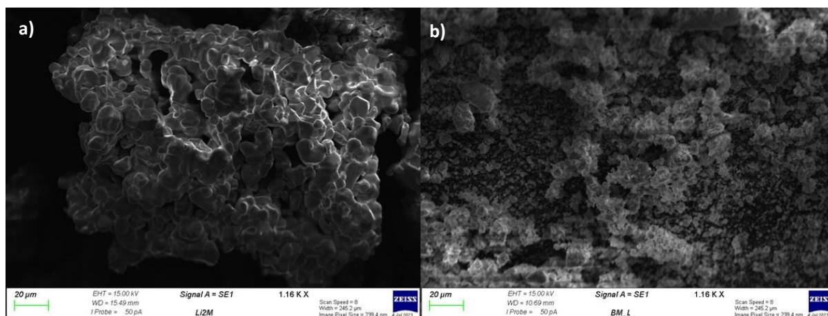
Figure 5: SEM images of \text{Li}_2\text{MoO}_4 - pristine (a) and ball milled (b).
