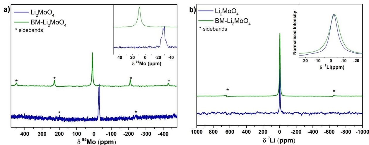
Figure 3: a) ^{95}\text{Mo} NMR for \text{Li}_2\text{MoO}_4 and \text{BM-Li}_2\text{MoO}_4 at 700 MHz (16.4 Tesla), 10 kHz MAS, single pulse spectra. b) ^7\text{Li} NMR at 200 MHz (4.7 Tesla), 50 kHz MAS, with 1 \mu\text{s} pulse for \text{Li}_2\text{MoO}_4 and \text{BM-Li}_2\text{MoO}_4 . In both figures, inset focuses on the central transition peak.
