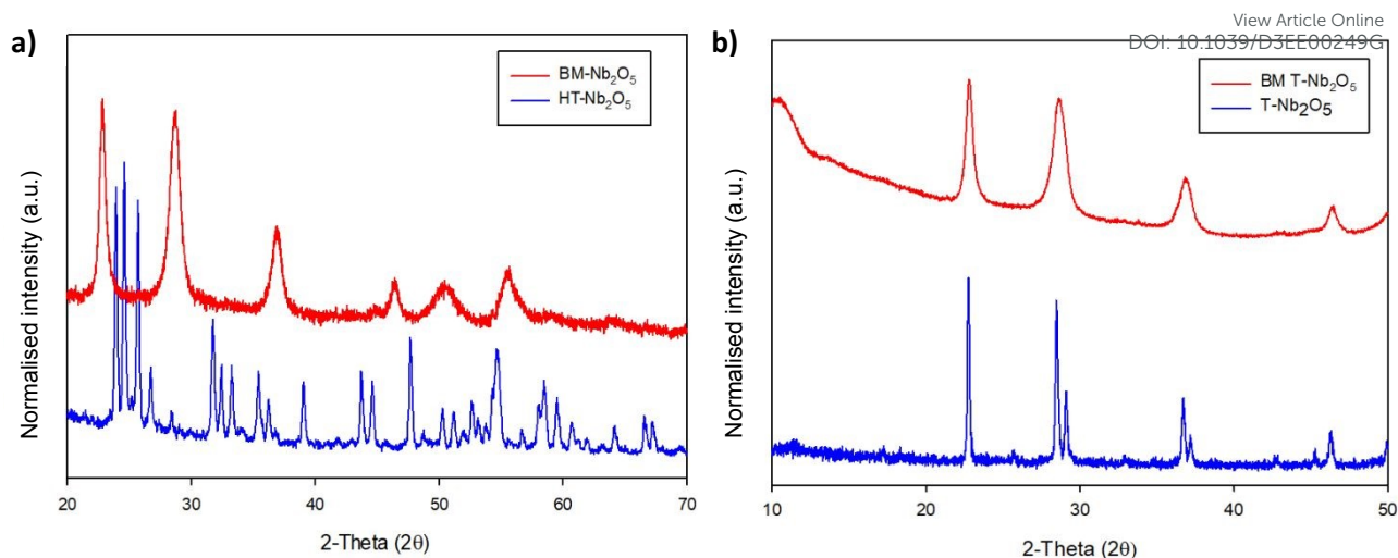
Figure 14: a) High temperature (HT) phase – H\text{-Nb}_2\text{O}_5 before and after milling (BM) showing a phase conversion to T\text{-Nb}_2\text{O}_5 . b) Low temperature phase ( T\text{-Nb}_2\text{O}_5 ) before and after milling showing no change in structure, just broadening of the peaks due to the smaller particle size after milling. (Cu K\alpha ).
