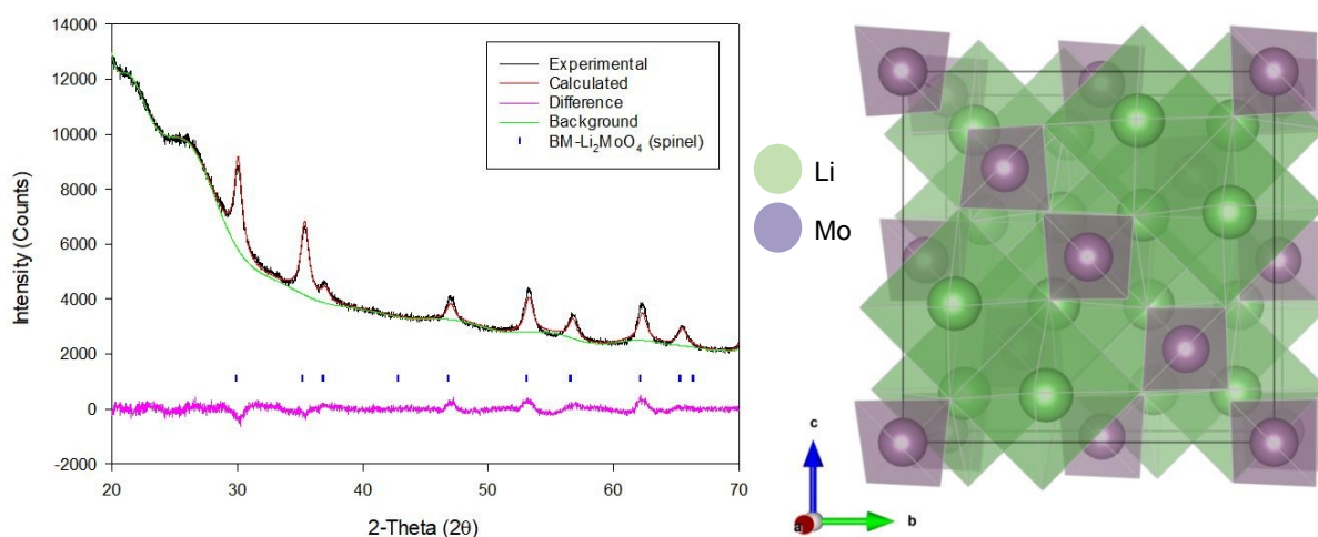
Figure 2: Observed, calculated and difference profiles for Rietveld refinement of BM-Li_2MoO_4 (16 h) (left) and an image of the spinel structure adopted by this phase (right). (Cu K\alpha ).
