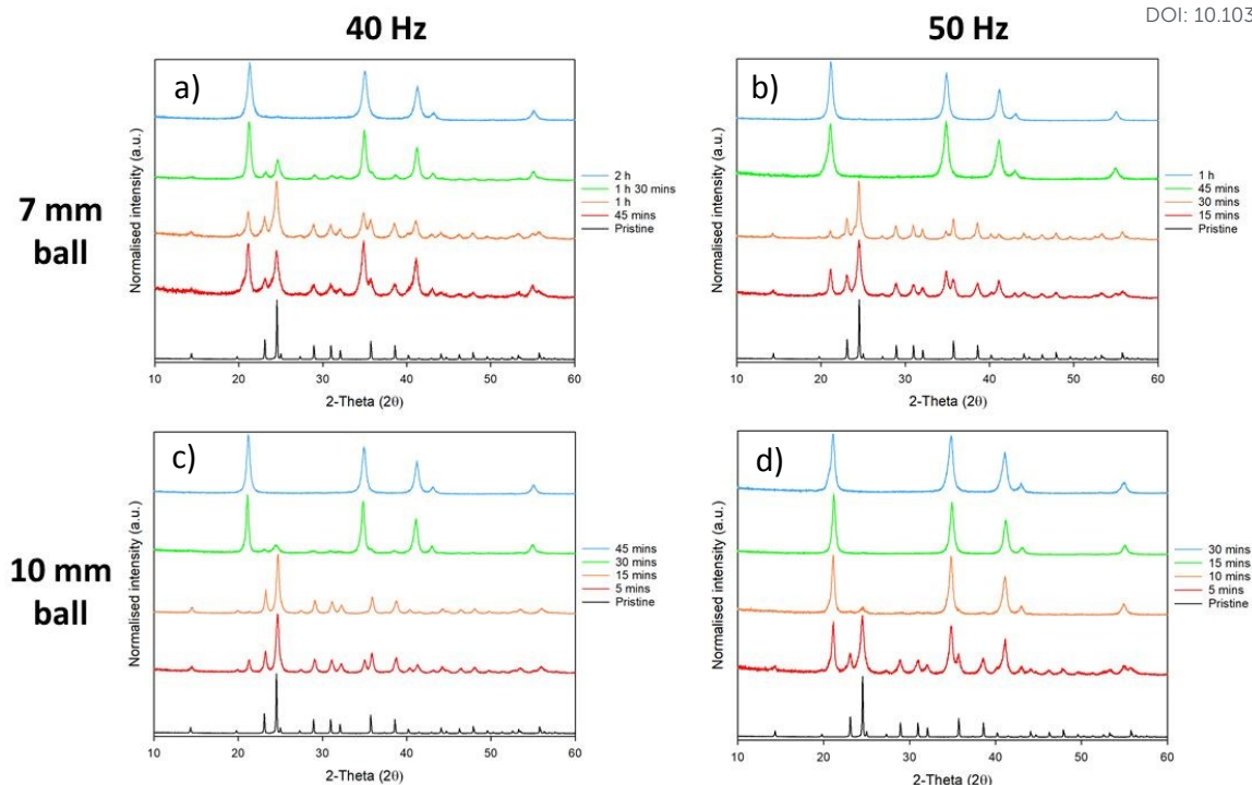
Figure 6: Resulting PXRD patterns from the study on ball mill frequency, time and ball size on the milling of \text{Li}_2\text{MoO}_4 . Patterns a) and b) made use of a 7 mm ball at 40 Hz and 50 Hz, respectively. Patterns c) and d) made use of a 10 mm ball at 40 Hz and 50 Hz respectively. The conversion rate was shown to significantly reduce through reducing the frequency and the ball size. (Co \text{K}\alpha ). 50 mg of material was loaded into the pots.
