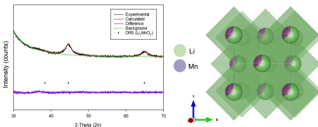
Figure 10: Observed, calculated and difference plot from the Rietveld refinement of BM- \text{Li}_2\text{MnO}_3 after 16 h (Cu \text{K}\alpha ) and an image of the crystal structure.
