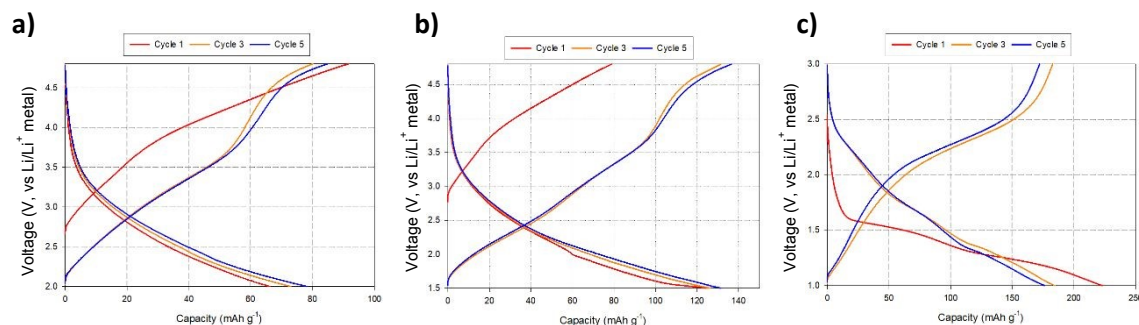
Figure 8: Voltage profiles for BM-Li 2 MoO 4 using varying voltage ranges: a) 4.8 - 2.0 V, b) 4.8 - 1.5 and c) 3.0 - 1.0 V.
