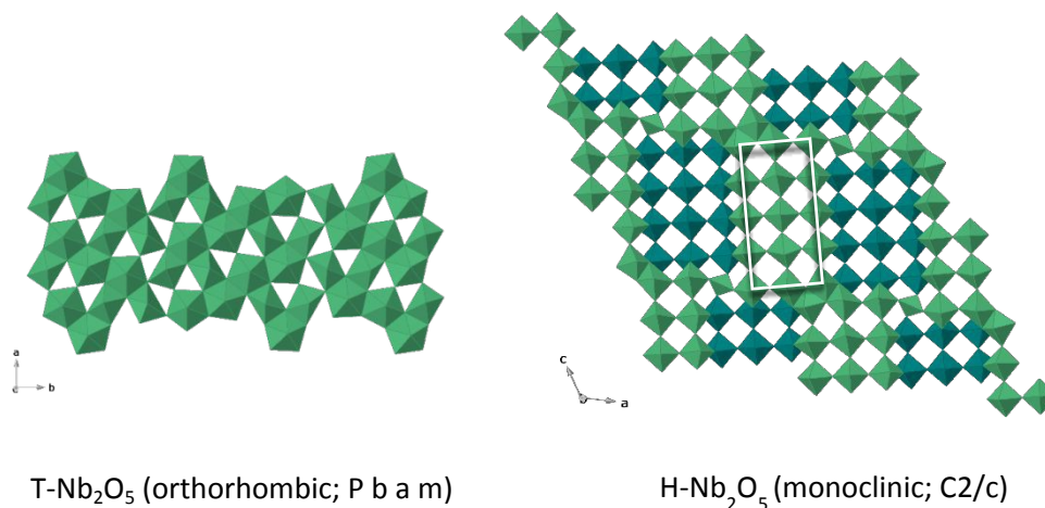
Figure 13: Crystal structures of T- and H-Nb 2 O 5 phases, left and right respectively. The Nb is represented by the polyhedra; for simplicity the oxygens have been omitted.
