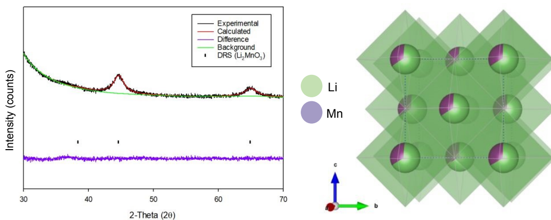
Figure 10: Observed, calculated and difference plot from the Rietveld refinement of \text{BM-Li}_2\text{MnO}_3 after 16 hours ( \text{Cu K}\alpha ) and an image of the crystal structure.
