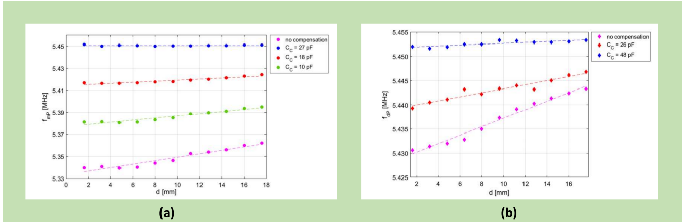
FIGURE 10. (a) Measurement of the maximum real part of Re\{Z_1\} for different wireless interrogation distance without using capacitance compensation circuit indicating as no compensation and with capacitance compensation circuit in parallel to the readout coil as indicated C_c [65], (b) measurement of the damped decay response for different wireless distances without capacitance compensation circuit indicating no compensation and with a capacitance compensation circuit indicating C_c [65].
