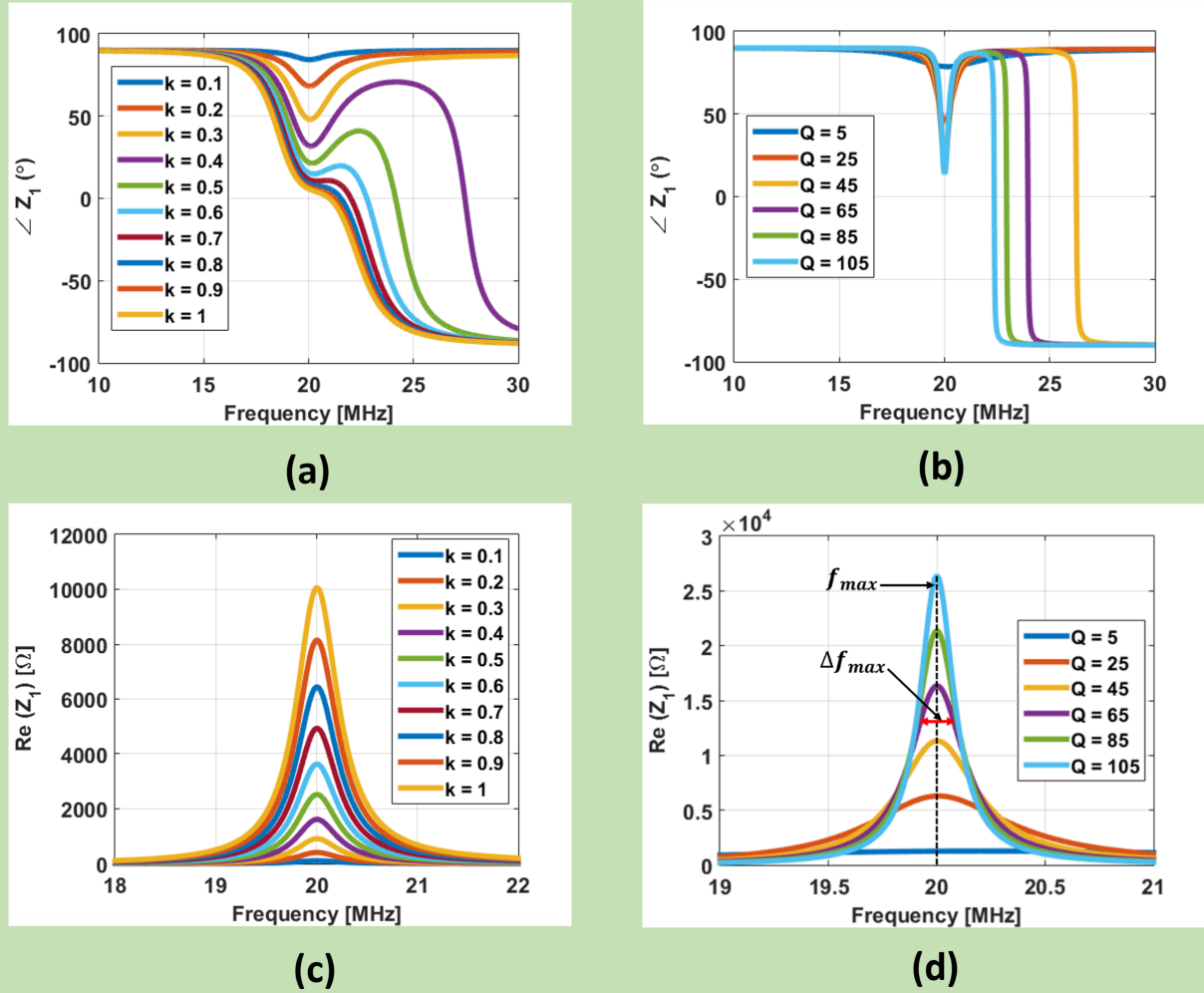
FIGURE 5. (a) Simulated equivalent impedance phase as a function of frequency for different values of coupling coefficient k [59], (b) the effect of different values of quality factor Q on the impedance phase, (c) maximum real part of the equivalent impedance as a function of frequency for different values of k [59], (d) the effect of different values of Q on the maximum real part of the equivalent impedance.
