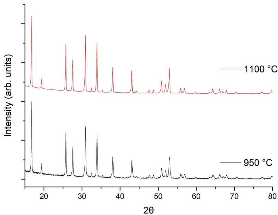
Figure 1. XRD patterns of LTC sintered in powder form (950°C, 100°C min -1 ) and as a pellet (1100°C, 40°C min -1 ). Both samples were sintered for 1h and demonstrate pure garnet ( Ia \bar{3}d ) type symmetry. In both cases heating rates were the maximum available for the furnace model.
