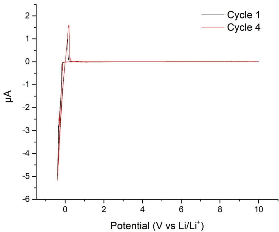
Figure 6. Cyclic voltammetry of LTC at room temperature using an Au/LTC/Li cell.
