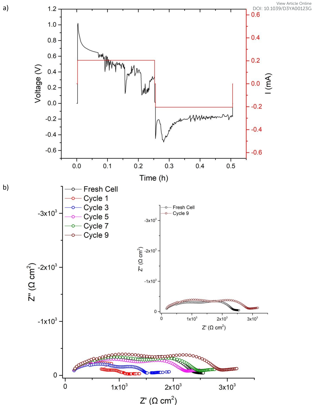
Figure 8. Results for the LTC cell was cycled at 500 \mu\text{A cm}^{-2} for a) one cycle with the corresponding impedance analysis in b). Cycle 1 was taken 2 minutes after, as sample needed to be transported to the Solartron impedance analyser to collect data. Time difference between subsequent impedance cycles is 3 minutes, which is the length of each scan. Time difference between cycle 7 and 9 is 90 minutes.
