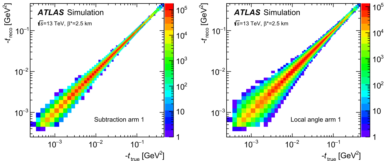
Fig. 13 The migration matrix of the t -value at reconstruction and generation level in Arm 1 for the subtraction and local angle methods
