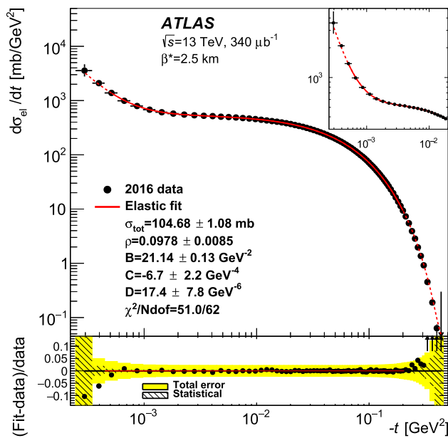
Fig. 19 A fit of the BCD -model with \sigma_{\text{tot}} , \rho , B , C and D as free parameters to the differential elastic cross section reconstructed with the subtraction method. The red full line represents the result of the fit inside the fit range, the dotted red line shows the extrapolation of the fit outside, including a special model for large |t| matched to the fitted function at -t = 0.2 \text{ GeV}^2 . In the lower panel, the points represent the deviation from unity of the ratio of the fit to the data, the yellow area represents the total experimental uncertainty and the hatched area the statistical component. The arrows indicate points out of the scale. The inset plot shows a zoom in the small- |t| region
