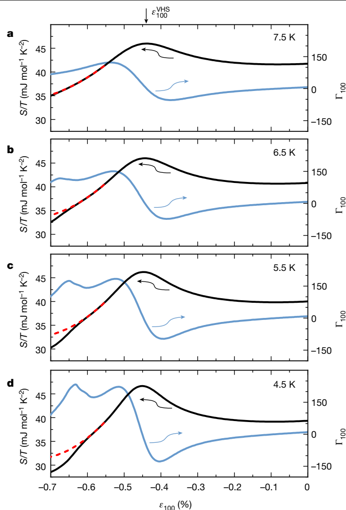
Fig. 4 | Strain dependence of the entropy. a–d, Integrating the \Gamma_{100} data using the iterative procedure described in Methods yields the strain-dependent entropy, plotted as S/T (black line) and directly compared with the measured \Gamma_{100} (blue line). The peak in \Gamma_{100} and corresponding rapid decrease of S/T indicates the magnetic transition at 4.5 K, 5.5 K and 6.5 K (b–d), whereas no decrease is visible at 7.5 K (a). The dotted red lines in the entropy traces are extrapolations of the background S/T from -0.55\% to a lower cut-off consistent with the varying onset of the magnetic transition ( -0.58\% , -0.59\% , -0.60\% and -0.61\% for 4.5 K, 5.5 K, 6.5 K and 7.5 K, respectively).
