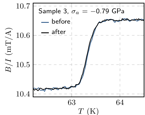
FIG. 6. Two measurements of sample 3 at \sigma_a = -0.79 GPa, before and after \sigma_a was ramped to -1.6 GPa.
