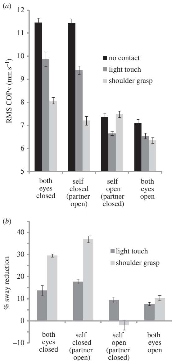
Figure 5. Effects of interpersonal touch and vision upon sway. Sagittal COPv is shown in (a) for all conditions. Percentage changes in sway relative to the NC condition are shown in (b). Bars show s.e.m.
