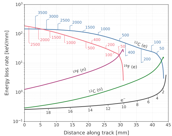
Fig. 2. Left — Track length in \text{CF}_4 at 50 Torr for electrons (mean projected range calculated with Degrad [48], CSDA range with ESTAR [51], and the practical range formula from Ref. [52], and mean projected range for carbon and fluorine ions from SRIM [49]). Right — Electronic and nuclear energy loss rates (CSDA) along carbon and fluorine ion tracks in \text{CF}_4 at 50 Torr, calculated with SRIM and electronic energy loss for 20 keV electrons obtained with ESTAR; called out values are interim particle energies (in keV) remaining at that point in the track.
