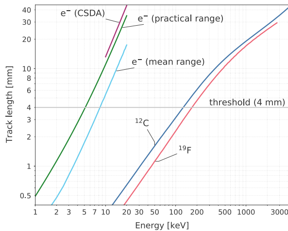
Fig. 2. Left — Track length in \text{CF}_4 at 50 Torr for electrons (mean projected range calculated with Degrad [48], CSDA range with ESTAR [51], and the practical range formula from Ref. [52], and mean projected range for carbon and fluorine ions from SRIM [49]). Right — Electronic and nuclear energy loss rates (CSDA) along carbon and fluorine ion tracks in \text{CF}_4 at 50 Torr, calculated with SRIM and electronic energy loss for 20 keV electrons obtained with ESTAR; called out values are interim particle energies (in keV) remaining at that point in the track.
