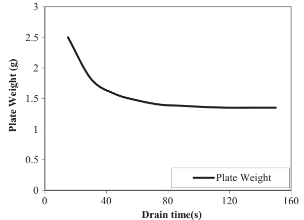
Fig. 2. The draining curve of zirconia slurry over initial 150 s.
